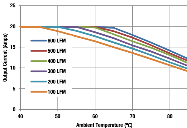
Figure 11 Maximum Current Derating (Vin = 160V)
