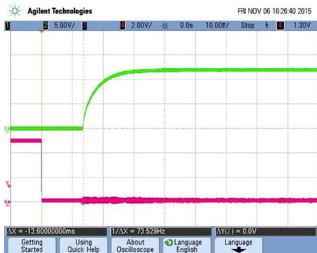
Figure 15: Turn-on transient at zero load current (10 mS/div, Top Trace: Vout, 5V/div; Bottom Trace: ON/OFF, 2V/div)
