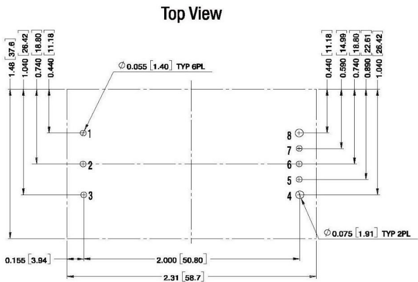
Recommended Footprint for Slotted / Flanged Baseplate
