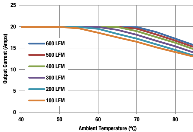
Figure 7 Maximum Current Temperature Derating (Vin = 57.6V)
