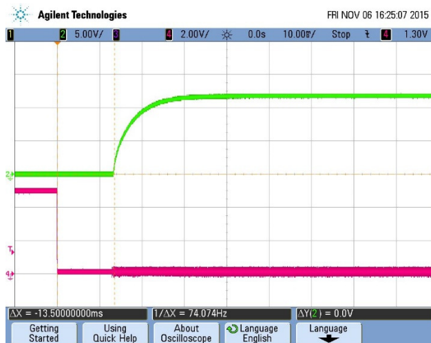
Figure 16: Turn-on transient at full load current (10 mS/div, Top Trace: Vout, 5V/div; Bottom Trace: ON/OFF, 2V/div)
