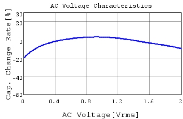
GRM21BR60J476ME01 C-AC Voltage capchange, D
