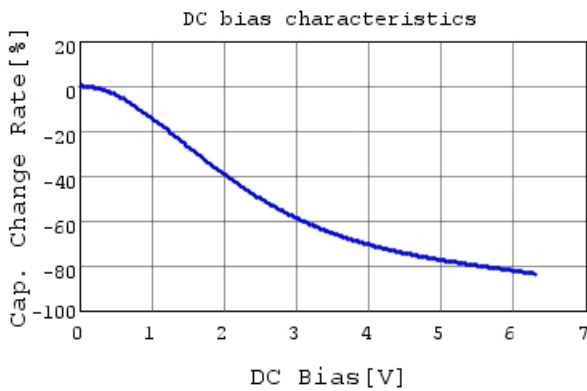
GRM21BR60J476ME01 C-DC bias capchange, 25.0C
