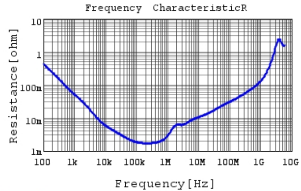
GRM21BR60J476ME01 R DCOV,25degC
