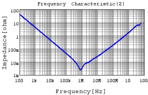
GRM21BR60J476ME01 |Z| DCOV,25degC
