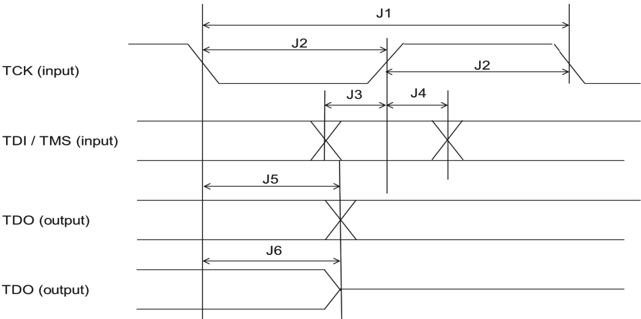
Figure 14. JTAG controller timing
