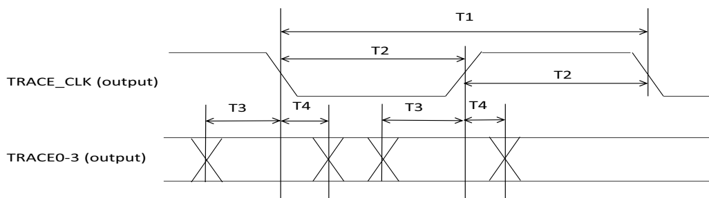
Figure 17. Trace timing
