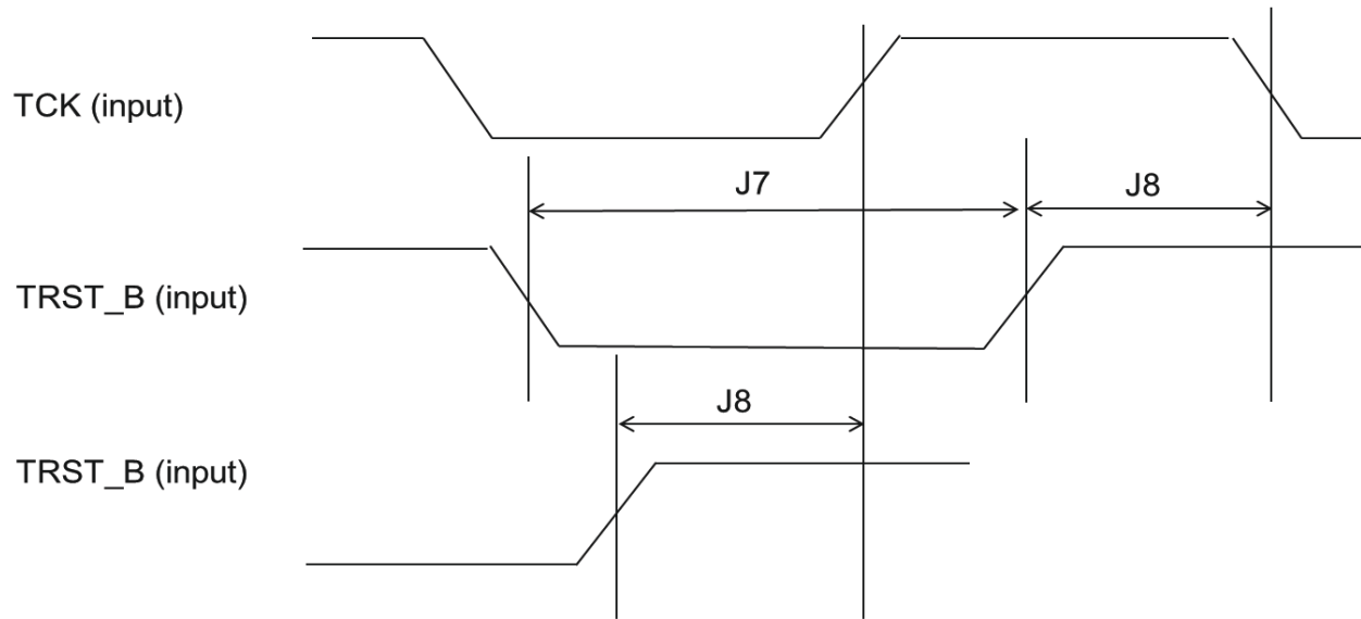
Figure 15. JTAG_TRST_B timing
