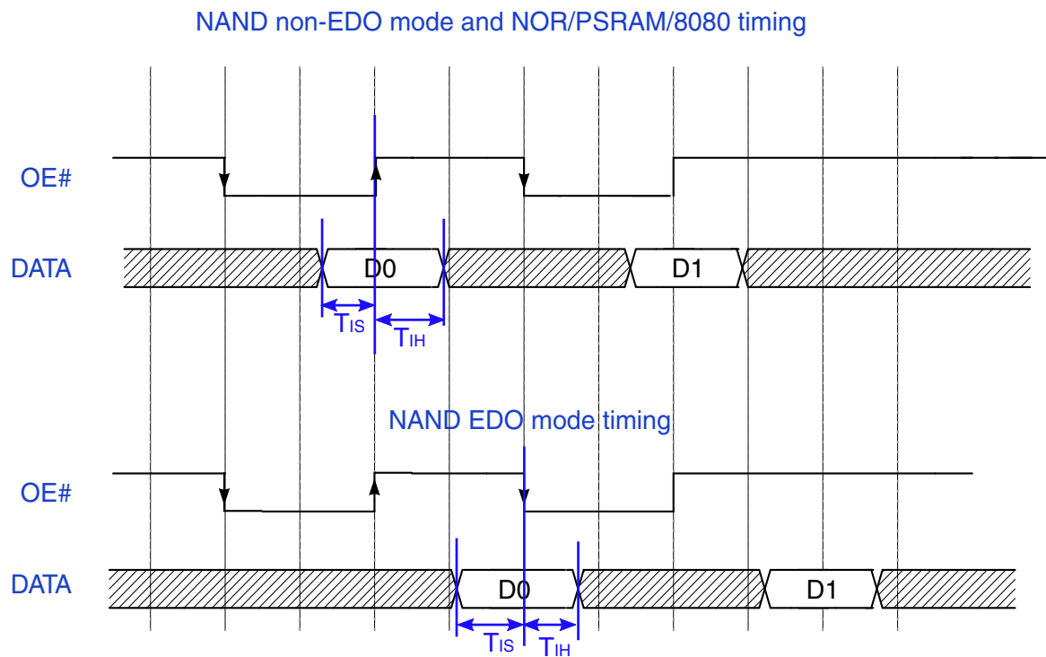
Figure 20. SEMC input timing in ASYNC mode
