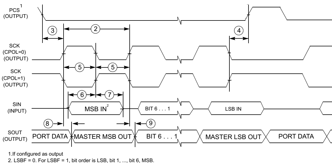
Figure 39. LPSPI Master mode timing (CPHA = 1)
