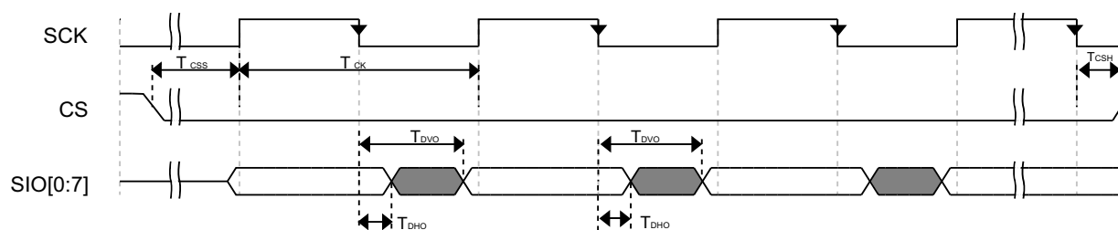
Figure 28. FlexSPI output timing in SDR mode
