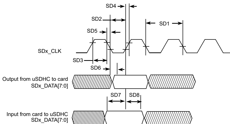
Figure 42. SD/eMMC4.3 timing
