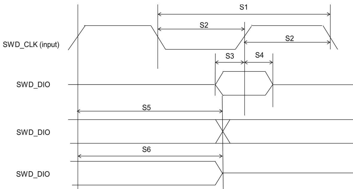
Figure 16. SWD timing
