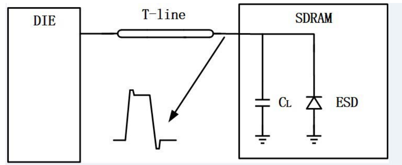
Figure 10. MCU-SDRAM circuit with overshoot/undershoot
