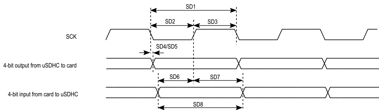
Figure 44. SDR50/SDR104 timing
