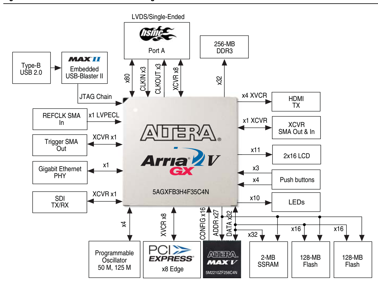
Figure 1-1. Arria V GX Starter Board Block Diagram
