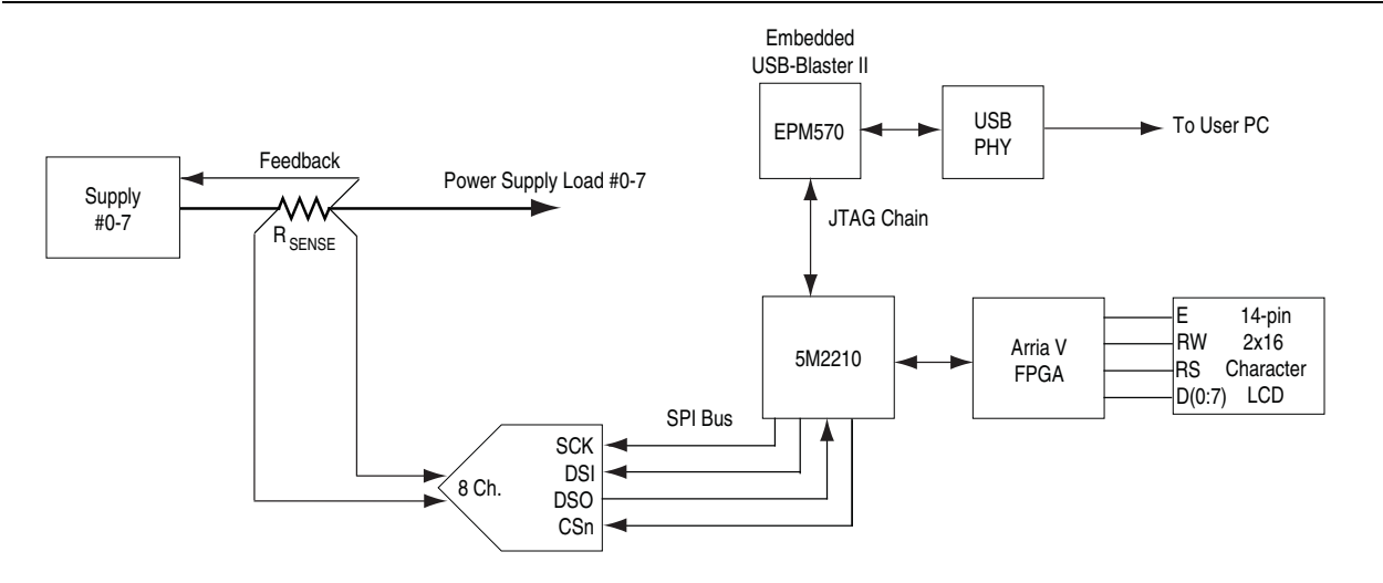
Figure 2-13. Power Measurement Circuit
