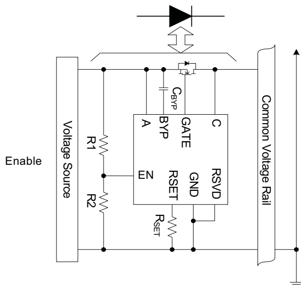
Figure 1. Typical Application
