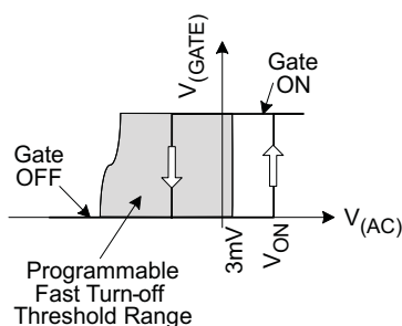
Figure 10. TPS2419 Operation
