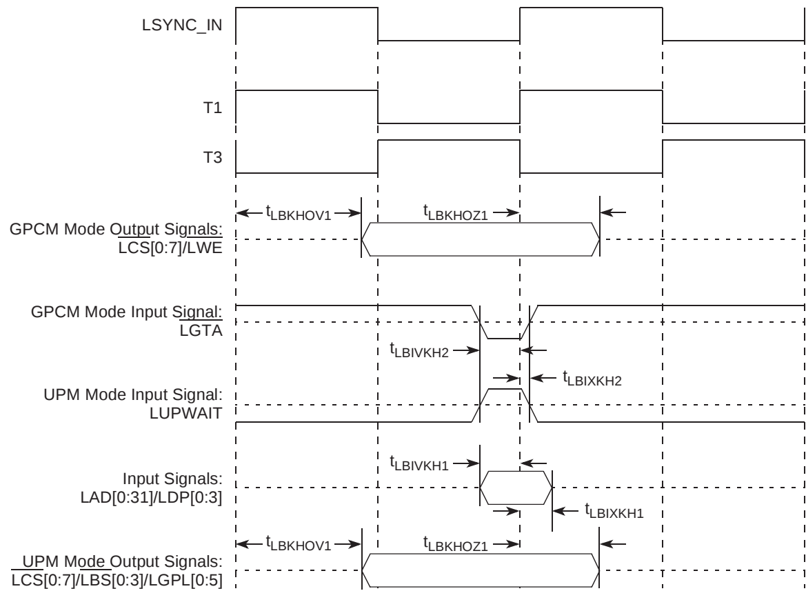
Figure 10-4. Local Bus Signals, GPCM/UPM Signals for LCCR[CLKDIV] = 4 (PLL Enabled)
