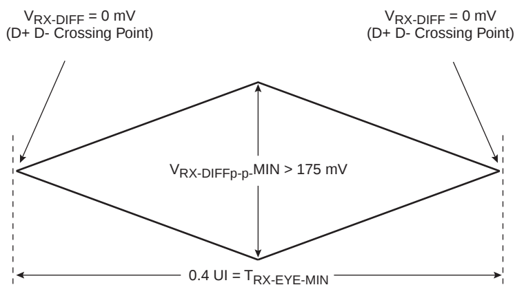
Figure 16-2. Minimum Receiver Eye Timing and Voltage Compliance Specification
