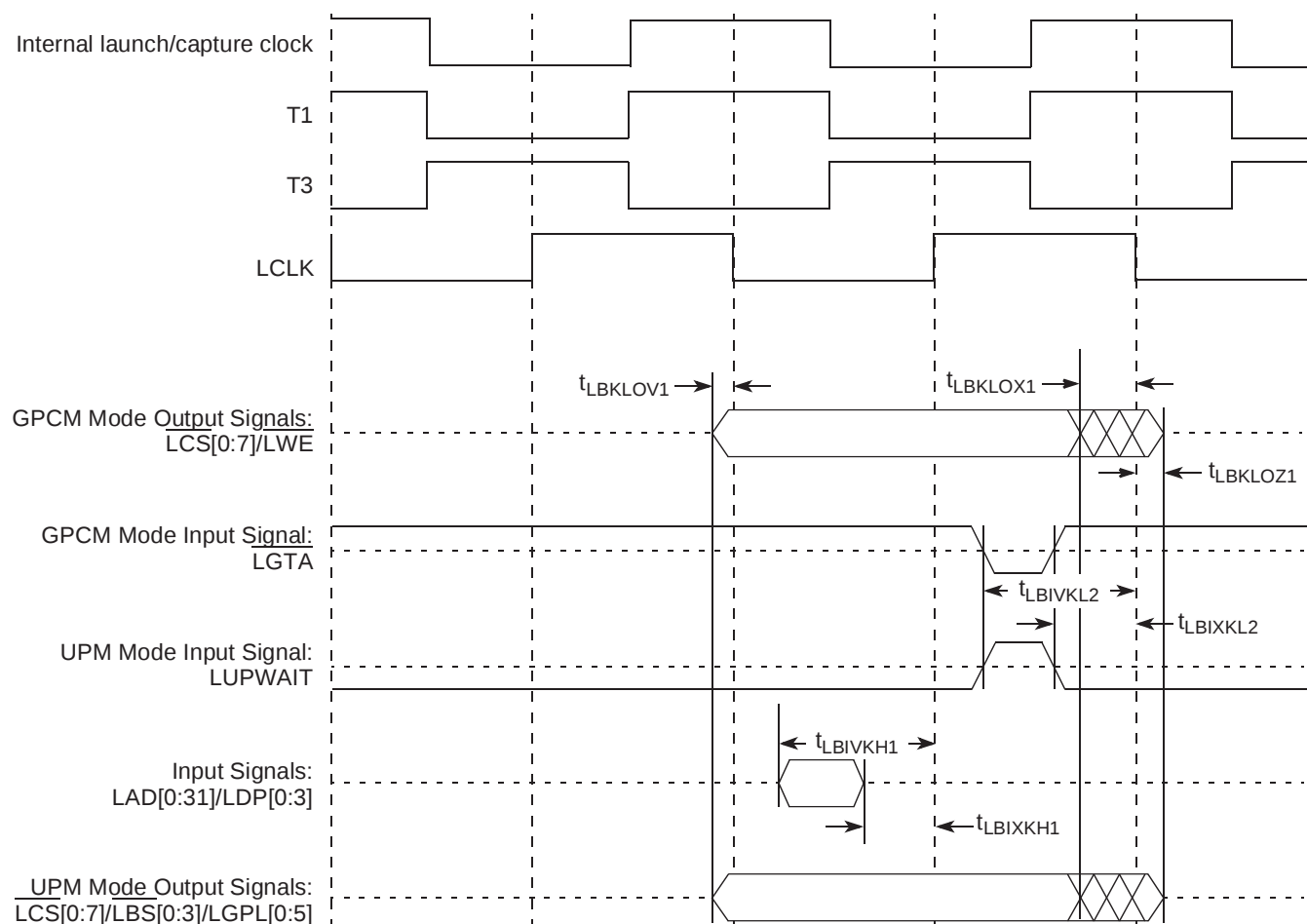
Figure 10-5. Local Bus Signals, GPCM/UPM Signals for LCCR[CLKDIV] = 4 (PLL Bypass Mode)
