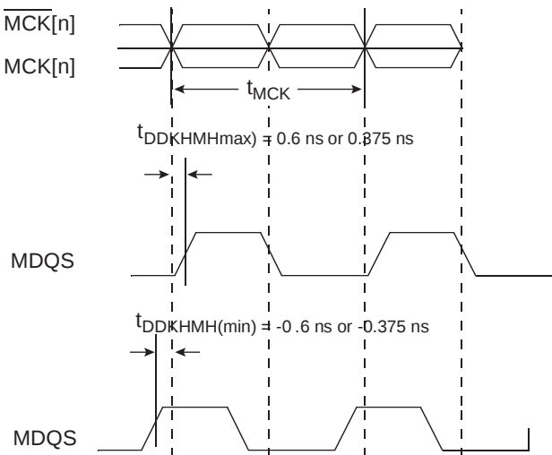
Figure 6-2. Timing Diagram for t_{DDKMH}
