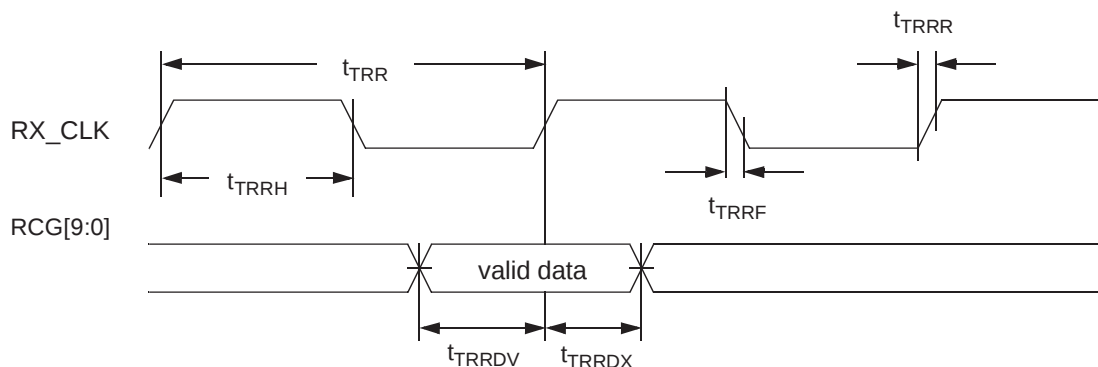
Figure 8-11. TBI Single-Clock Mode Receive AC Timing Diagram
