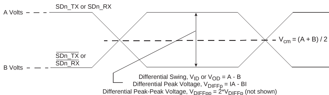
Figure 15-1. Differential Voltage Definitions for Transmitter or Receiver
