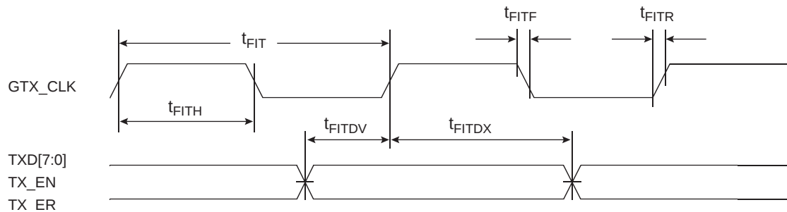
Figure 8-1. FIFO Transmit AC Timing Diagram
