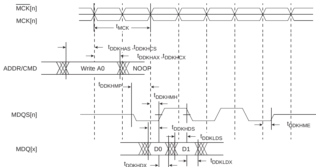
Figure 6-3. DDR2 and DDR3 SDRAM Interface Output Timing Diagram
