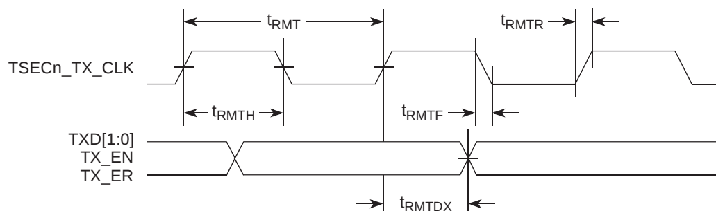
Figure 8-13. RMII Transmit AC Timing Diagram
