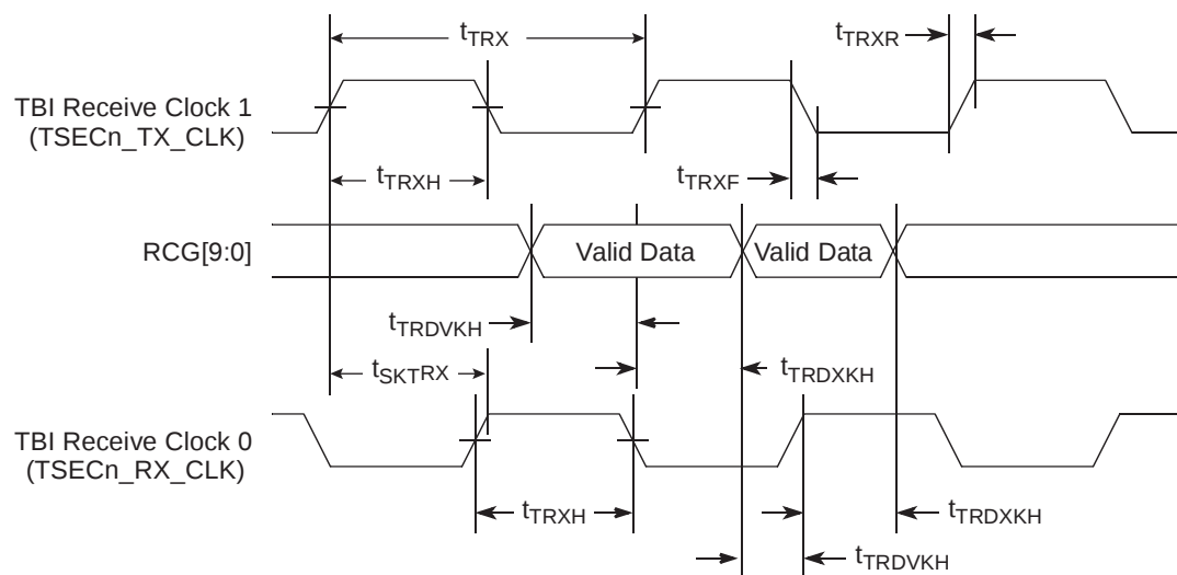
Figure 8-10. TBI Receive AC Timing Diagram
