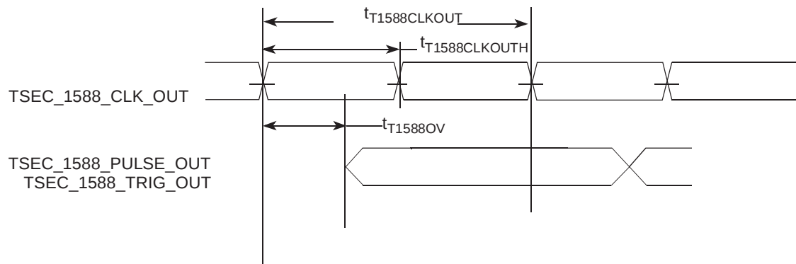
Figure 8-20. eTSEC IEEE 1588 Output AC Timing
