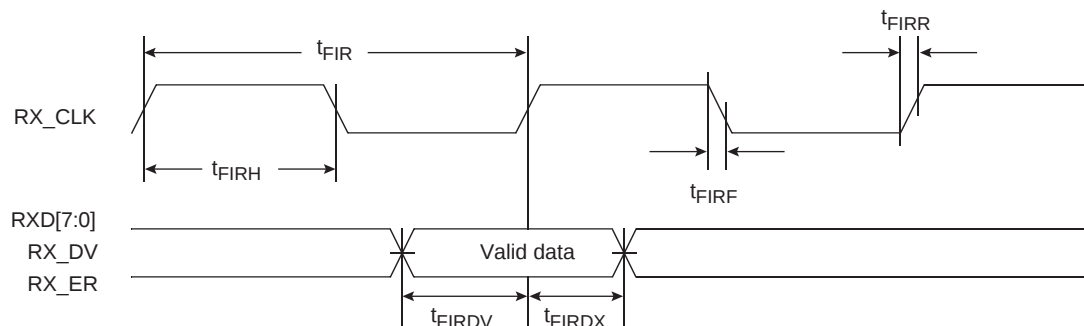
Figure 8-2. FIFO Receive AC Timing Diagram
