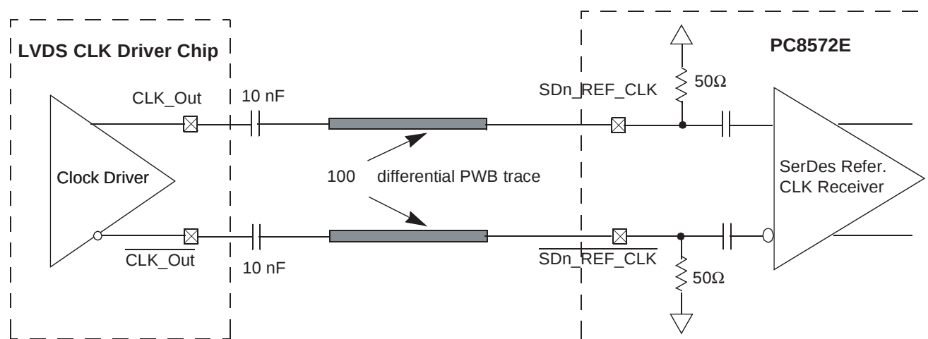
Figure 15-7. AC-Coupled Differential Connection with LVDS Clock Driver (Reference Only)
