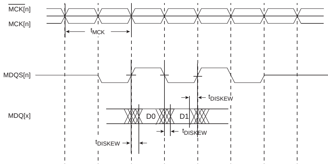
Figure 6-1. DDR2 and DDR3 SDRAM Interface Input Timing Diagram
