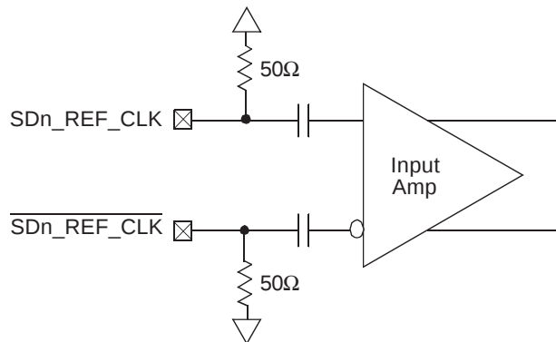
Figure 15-2. Receiver of SerDes Reference Clocks
