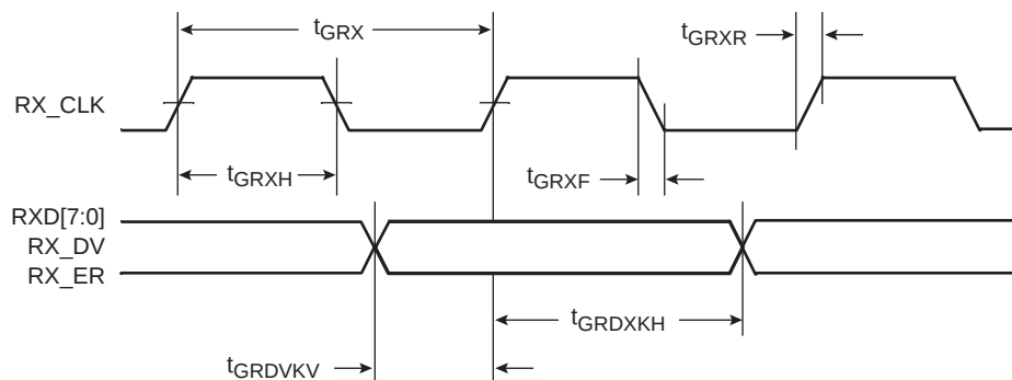
Figure 8-5. GMII Receive AC Timing Diagram
