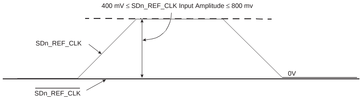
Figure 15-5. Single-Ended Reference Clock Input DC Requirements
