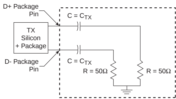
Figure 8-19. SGMII AC Test/Measurement Load
