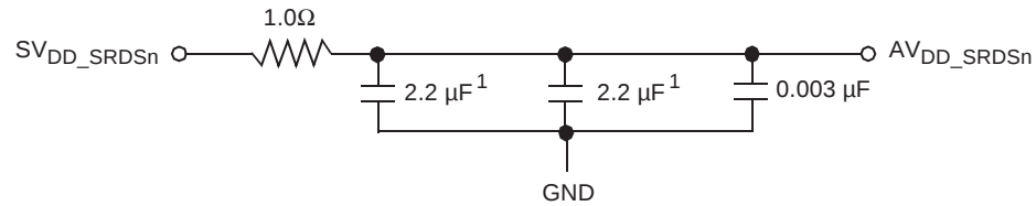
Figure 21-2. SerDes PLL Power Supply Filter
