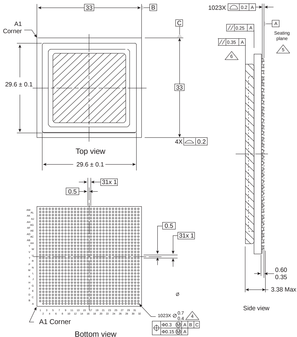
Figure 18-1. Mechanical Dimensions of the PC8572E FC-PBGA with Full Lid
