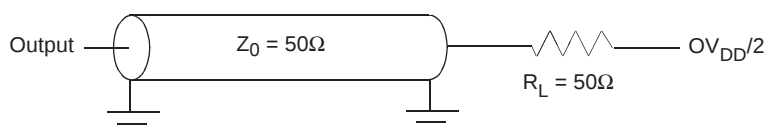
Figure 14-1. GPIO AC Test Load
