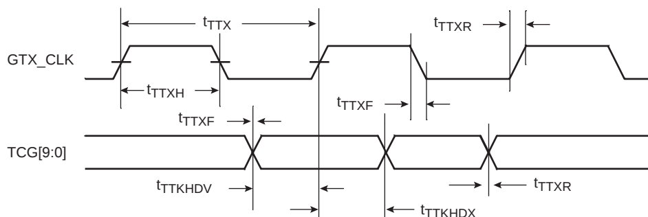
Figure 8-9. TBI Transmit AC Timing Diagram
