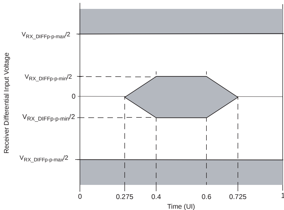
Figure 8-18. SGMII Receiver Input Compliance Mask
