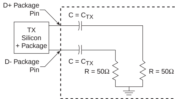
Figure 16-3. Compliance Test/Measurement Load
