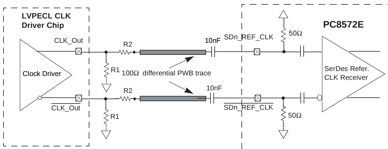
Figure 15-8. AC-Coupled Differential Connection with LVPECL Clock Driver (Reference Only)
