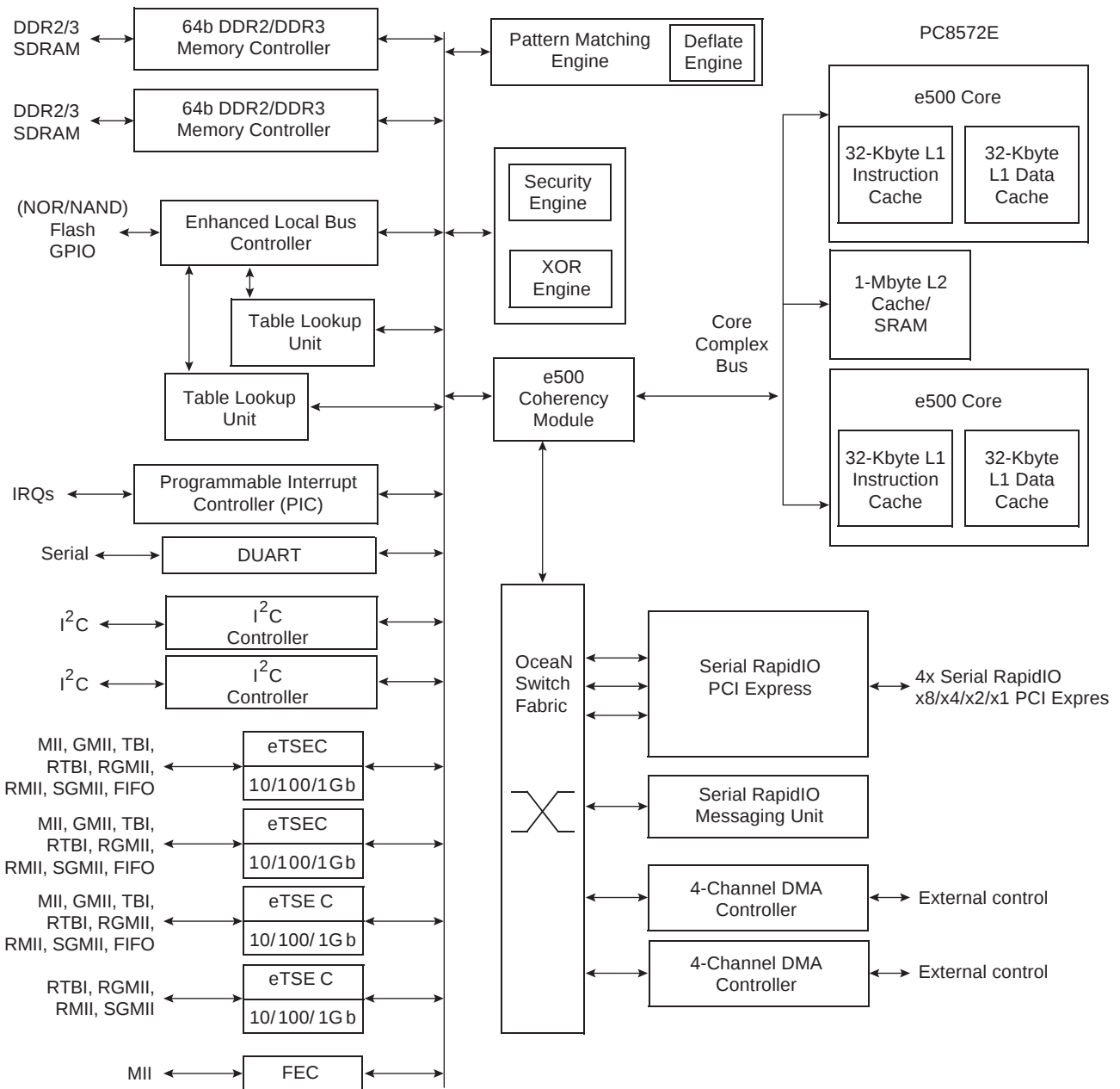
Figure 1-1. PC8572E Block Diagram
