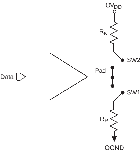
Figure 21-3. Driver Impedance Measurement
