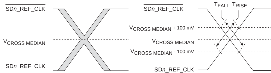
Figure 15-11. Single-Ended Measurement Points for Rise and Fall Time Matching
