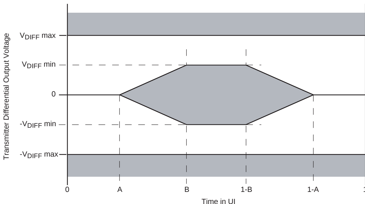
Figure 17-1. Transmitter Output Compliance Mask
