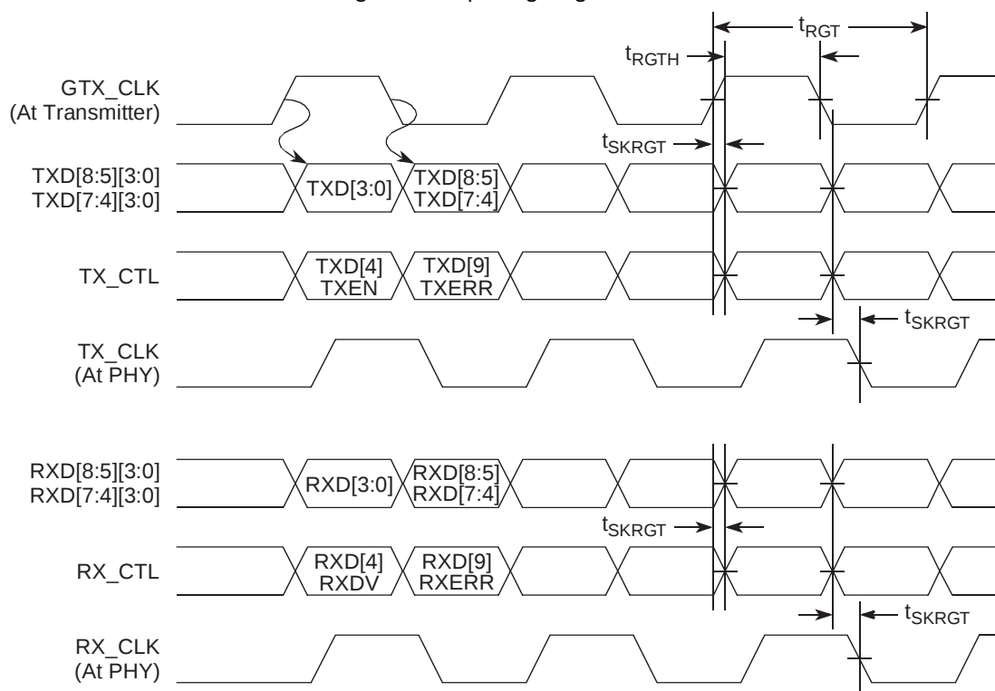
Figure 8-12. RGMII and RTBI AC Timing and Multiplexing Diagrams
