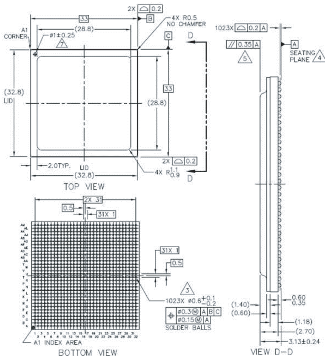
Figure 18-2. Mechanical Dimensions of the PC8572E FC-PBGA with stamp lid
