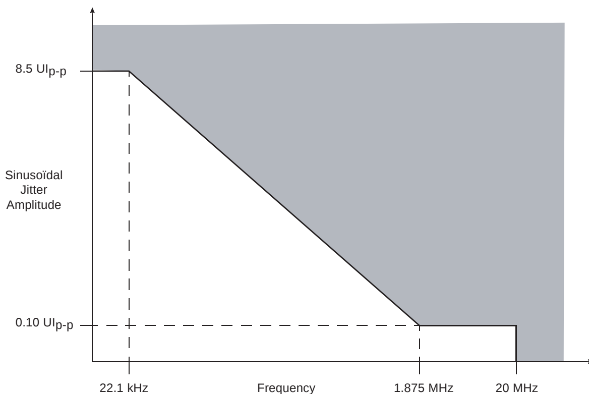
Figure 17-2. Single Frequency Sinusoidal Jitter Limits
