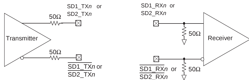
Figure 15-12. SerDes Transmitter and Receiver Reference Circuits
