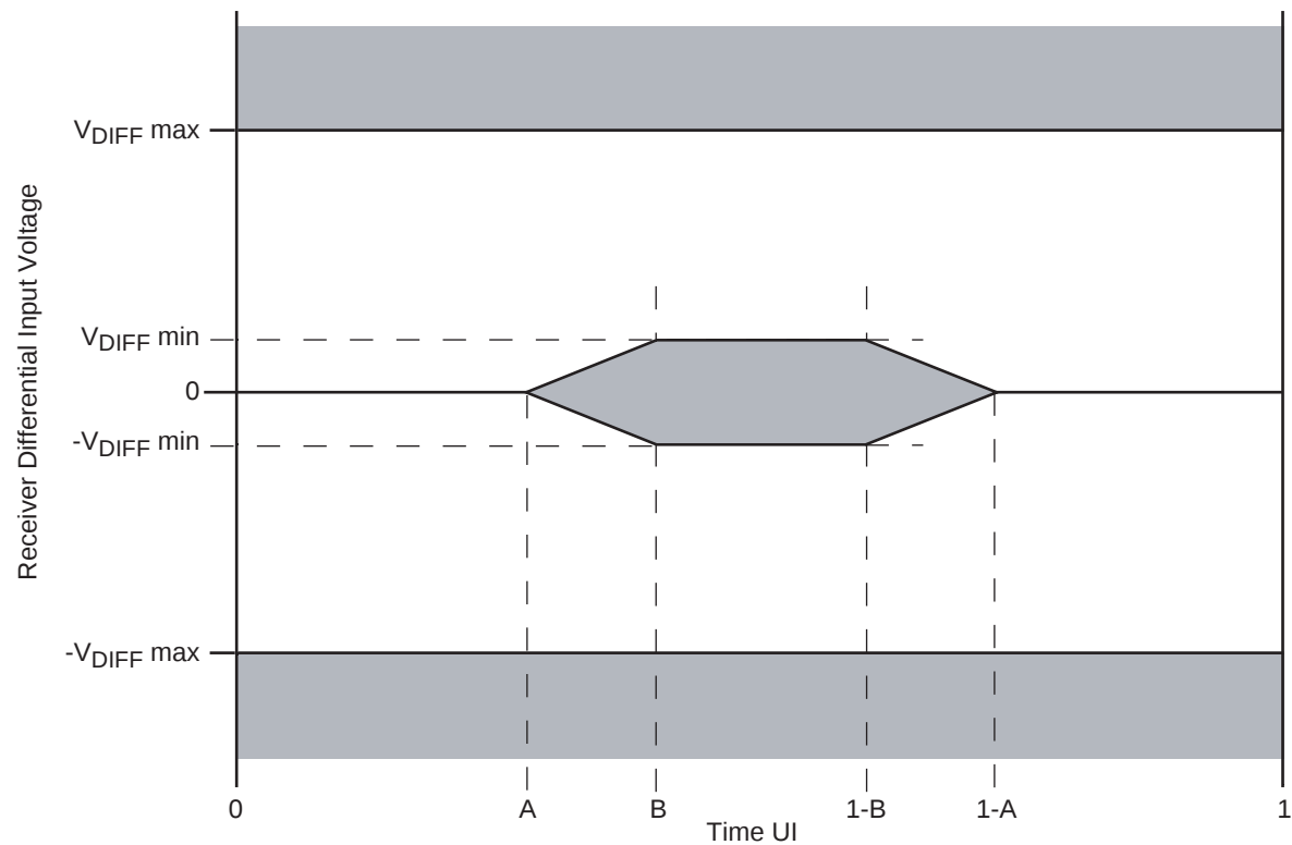
Figure 17-3. Receiver Input Compliance Mask
