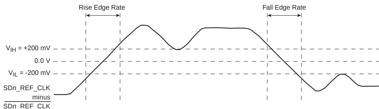
Figure 15-10. Differential Measurement Points for Rise and Fall Time
