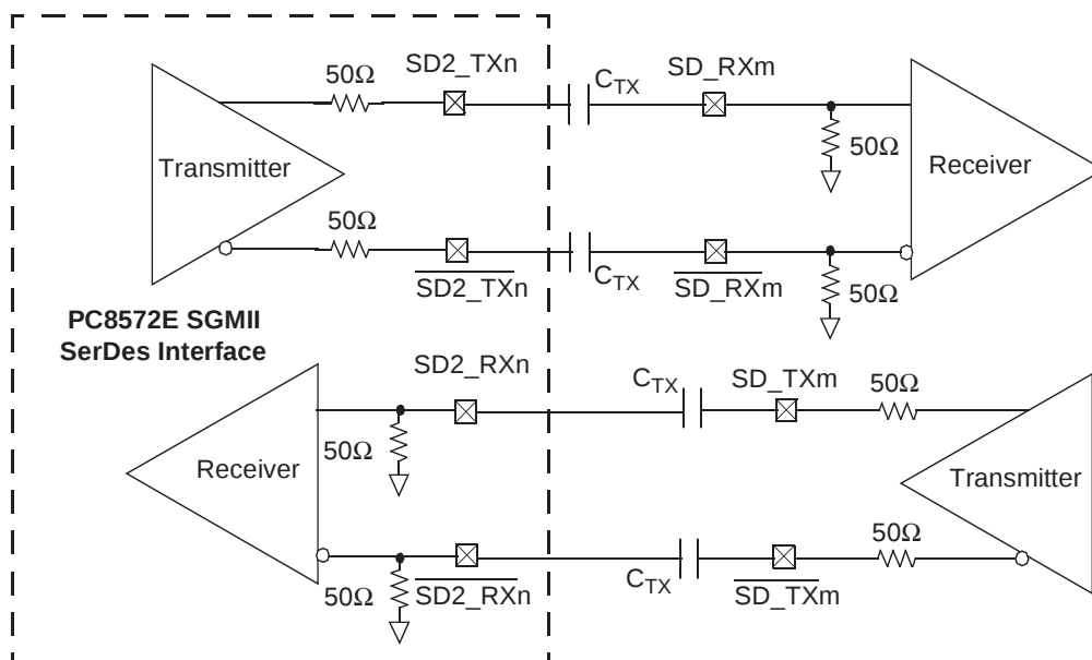
Figure 8-16. 4-Wire AC-Coupled SGMII Serial Link Connection Example
