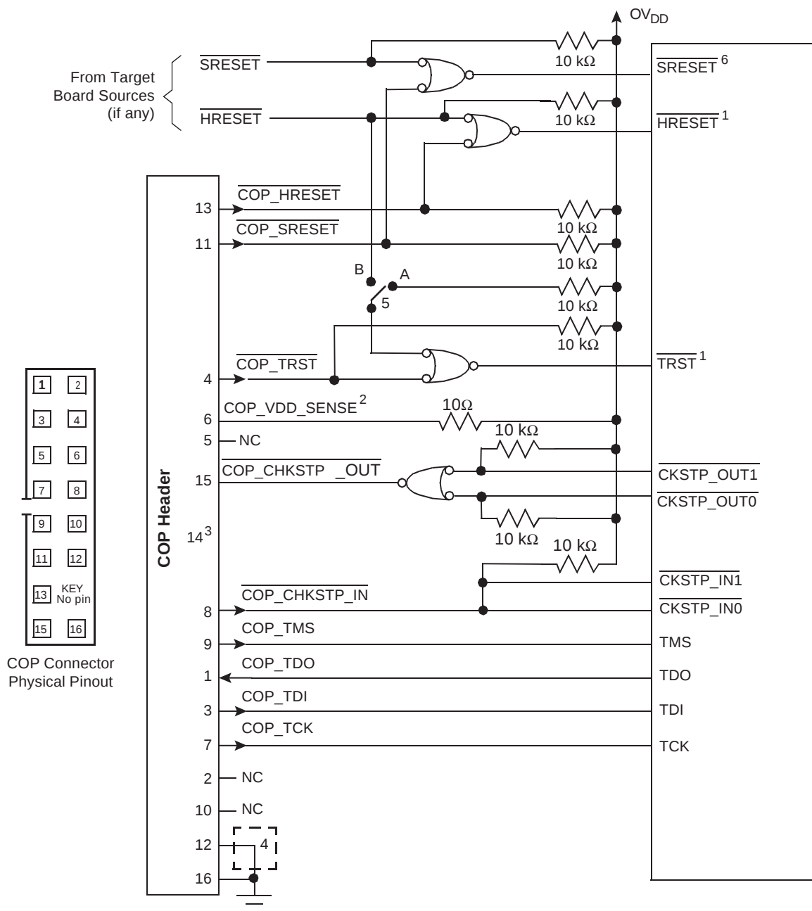
Figure 21-5. JTAG Interface Connection
