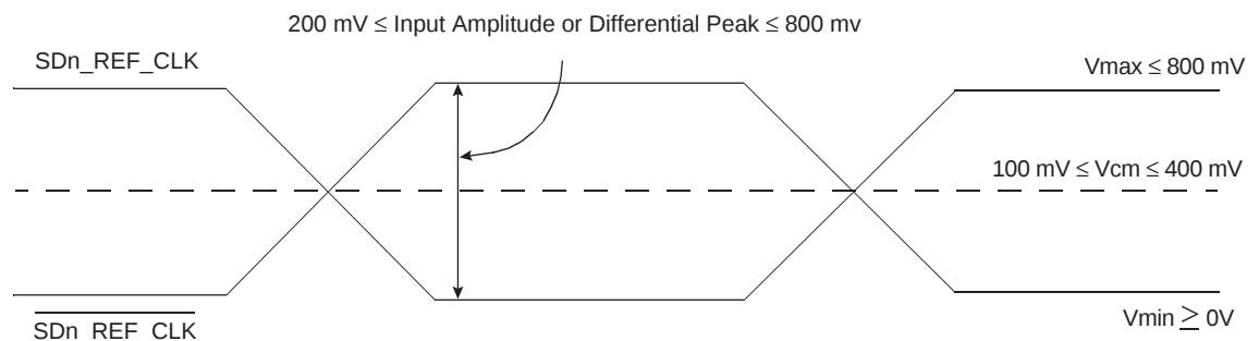
Figure 15-3. Differential Reference Clock Input DC Requirements (External DC-Coupled)
