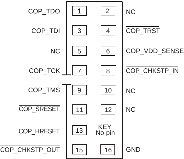
Figure 21-4. COP Connector Physical Pinout
