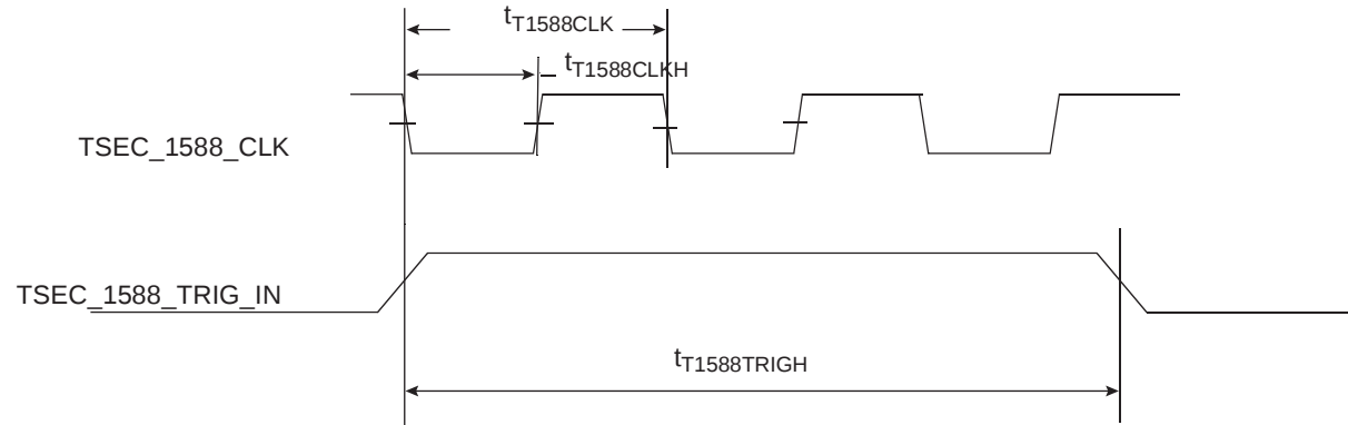
Figure 8-21. eTSEC IEEE 1588 Input AC timing
