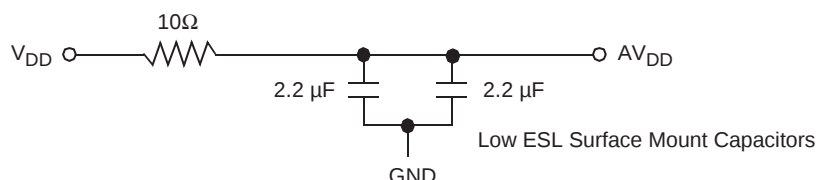
Figure 21-1. PLL Power Supply Filter Circuit
