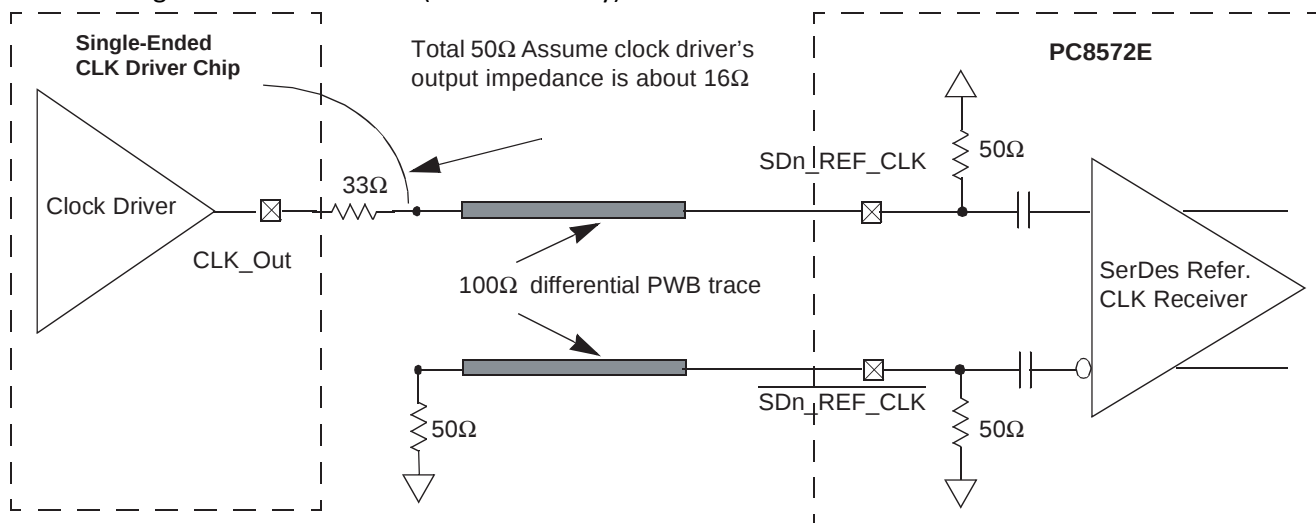
Figure 15-9. Single-Ended Connection (Reference Only)
