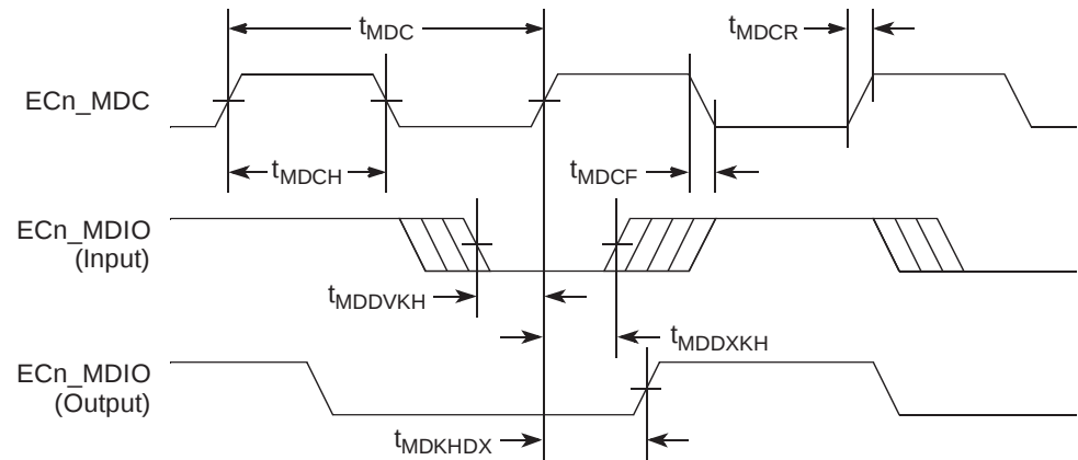
Figure 9-1. MII Management Interface Timing Diagram
