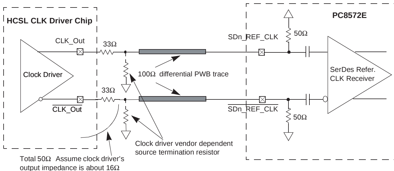
Figure 15-6. DC-Coupled Differential Connection with HCSL Clock Driver (Reference Only)
