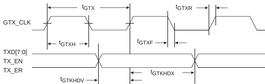
Figure 8-3. GMII Transmit AC Timing Diagram
