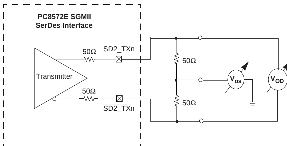
Figure 8-17. SGMII Transmitter DC Measurement Circuit
