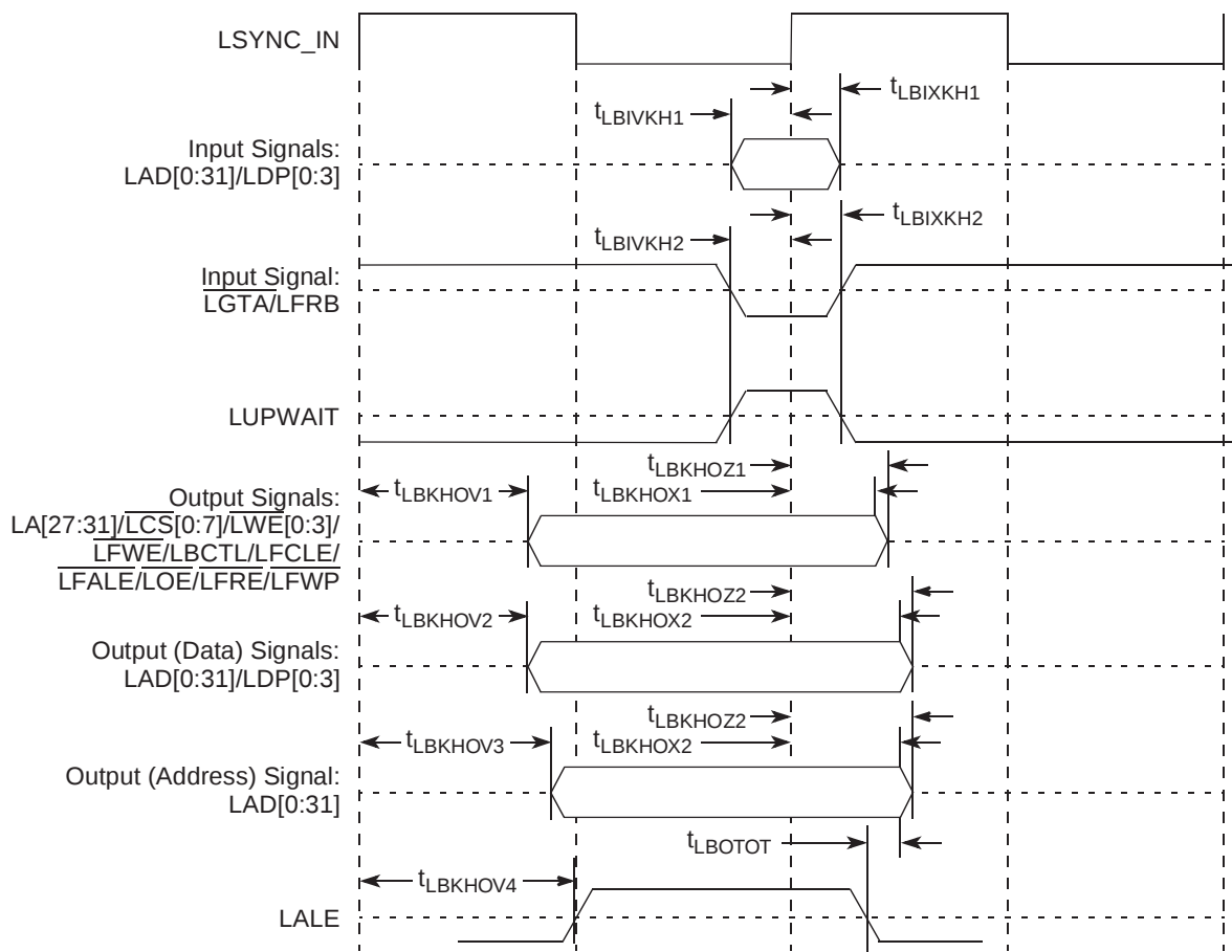
Figure 10-2. Local Bus Signals, Non-Special Signals Only (PLL Enabled)
