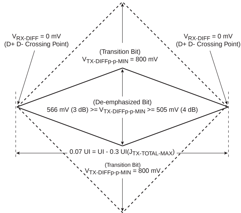
Figure 16-1. Minimum Transmitter Timing and Voltage Output Compliance Specifications
