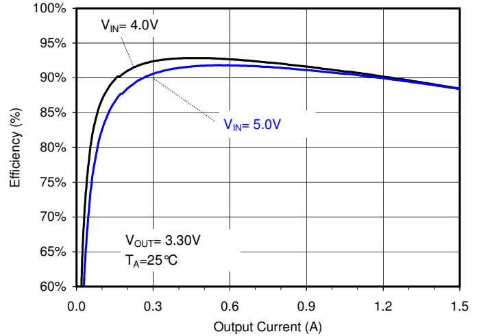
Efficiency vs. Load Current ( V_{OUT}=3.3V , SOT23-5)
