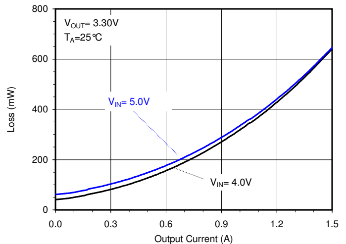
Total Loss vs. Load Current ( V_{OUT}=3.3V , SOT23-5)
