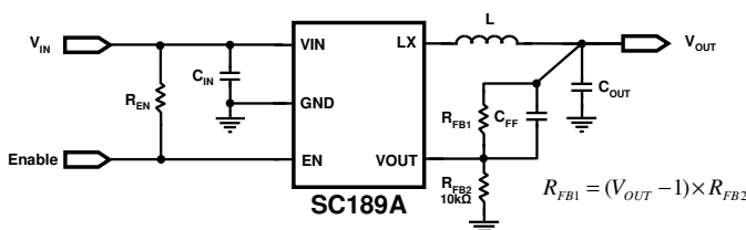
Figure 1 — Typical schematic for adjustable output voltage option from standard 1.0V of SC189A
