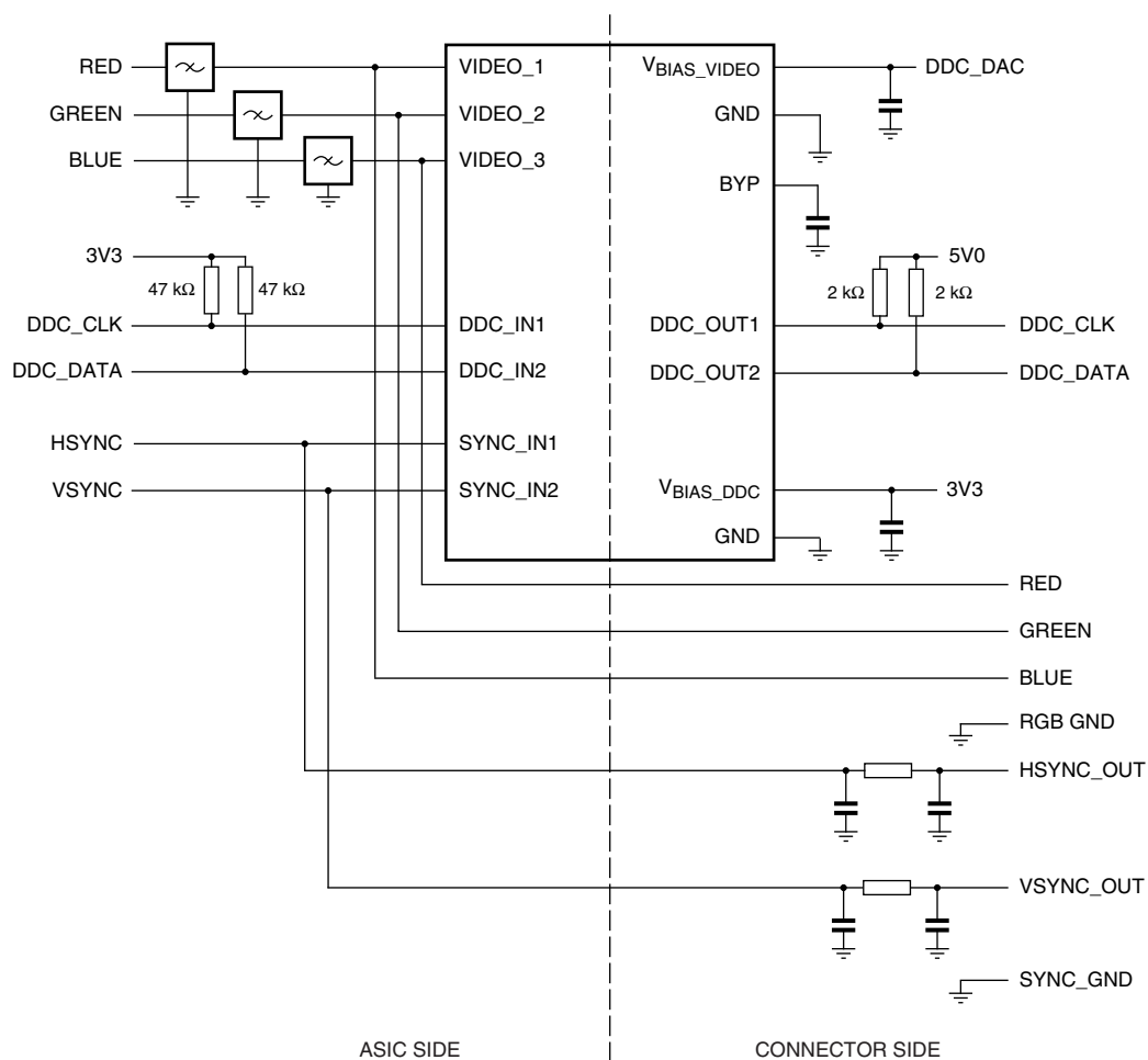
Fig 3. Application diagram
