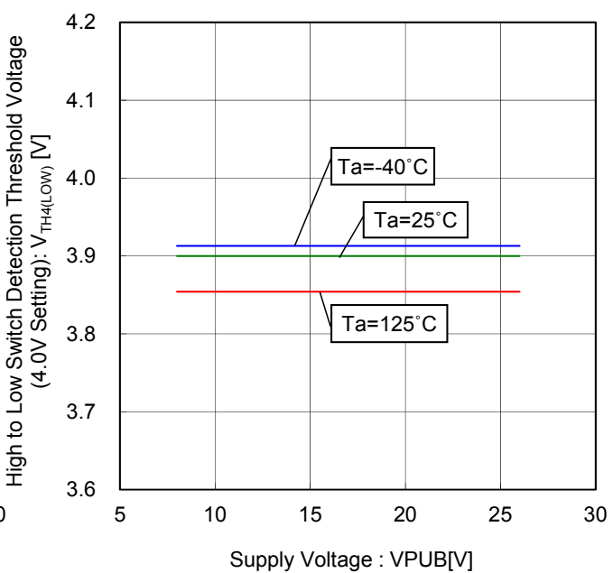
Figure 78. High to Low Switch Detection Threshold Voltage (4.0V Setting) vs Supply Voltage
