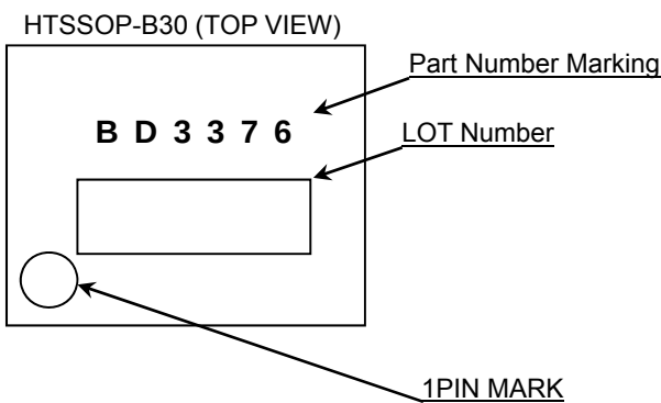
Figure 125. Marking Diagram
