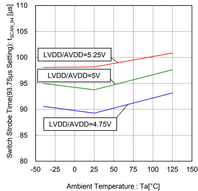
Figure 109. Switch Strobe Time(93.75µs Setting) vs Ambient Temperature
