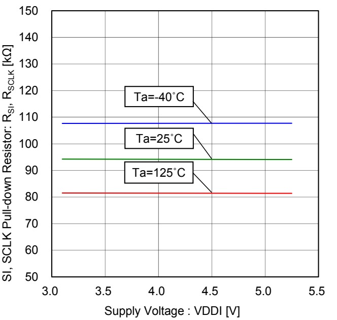
Figure 86. SI, SCLK Pull-down Resistor vs Supply Voltage
