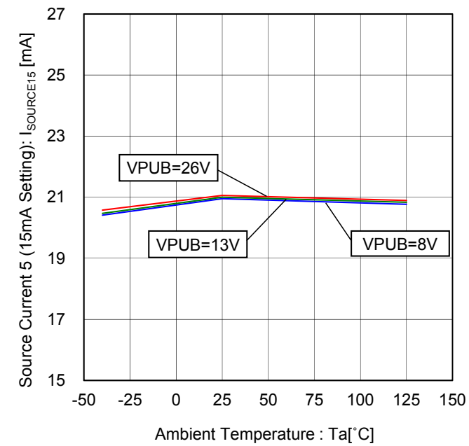
Figure 63. Source Current 5 (15mA Setting) vs Ambient Temperature (0V External Supply)
