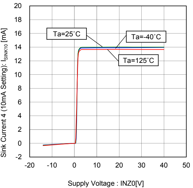
Figure 62. Sink Current 4 (10mA Setting) vs Supply Voltage
