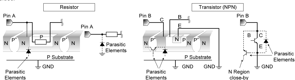
Figure 123. Example of monolithic IC structure
