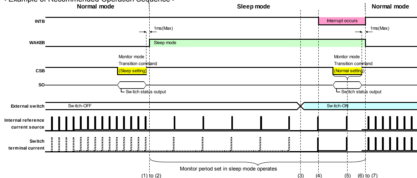
Figure 9. Basic Operation 3
