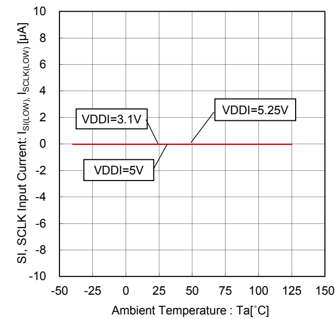
Figure 87. SI, SCLK Input Current vs Ambient Temperature (SI, SCLK=0V)
