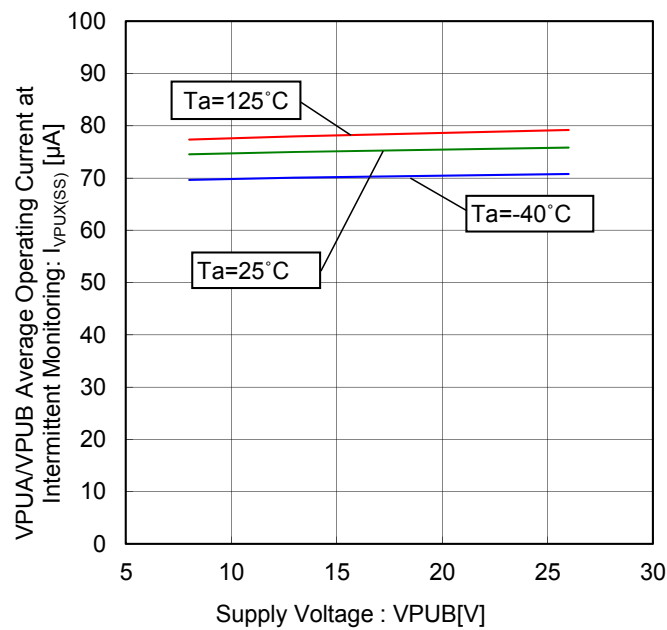
Figure 26. VPUA/VPUB Average Operating Current at Intermittent Monitoring vs Supply Voltage (Monitoring Period: 50ms, Strobe Time: 125 \mu s , Source/Sink Current Setting: 1mA)
