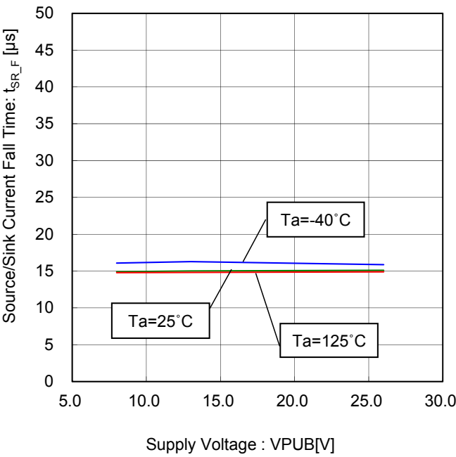
Figure 120. Source/Sink Current Fall Time vs Supply Voltage (FSQ="0", FSQZ/A/B="0", 10mA Setting, Load Resistance=100Ω)
