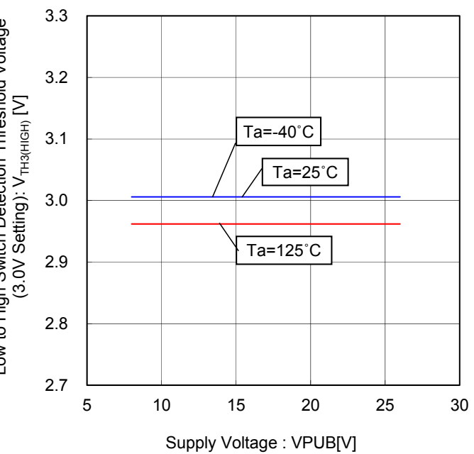
Figure 72. Low to High Switch Detection Threshold Voltage (3.0V Setting) vs Supply Voltage
