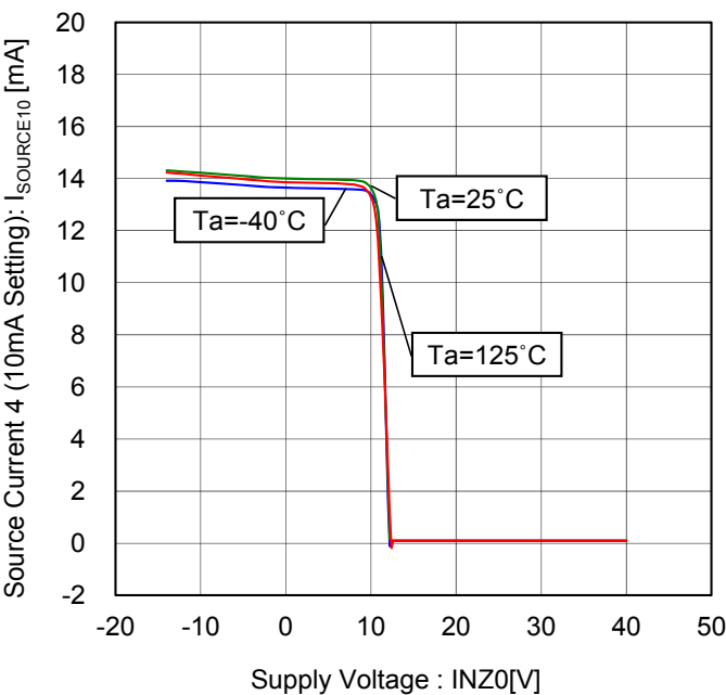
Figure 58. Source Current 4 (10mA Setting) vs Supply Voltage
