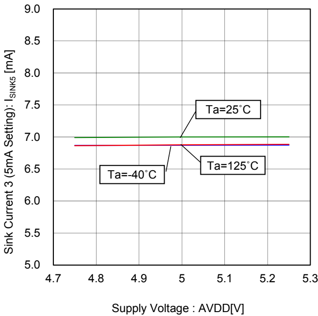
Figure 52. Sink Current 3 (5mA Setting) vs Supply Voltage (8V External Supply)
