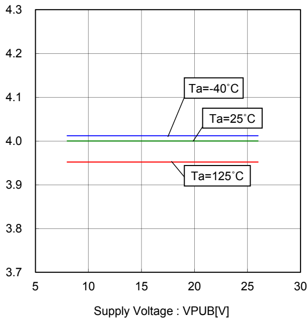
Figure 76. Low to High Switch Detection Threshold Voltage (4.0V Setting) vs Supply Voltage
