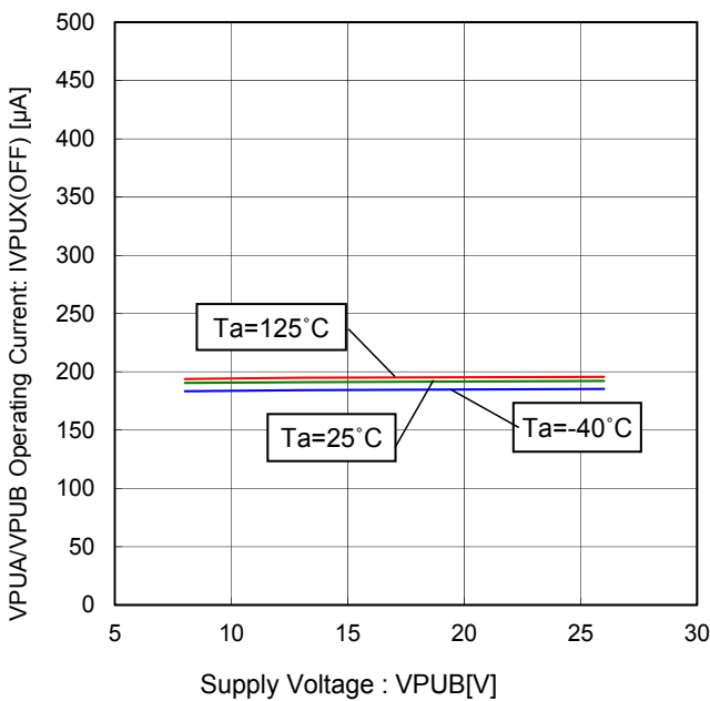
Figure 24. V_PUA/V_PUB Operating Current vs Supply Voltage (Continuous monitor setting, Current source is invalid, "Hi-Z" Status)
