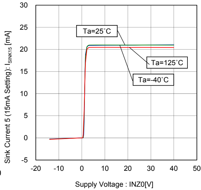
Figure 70. Sink Current 5 (15mA Setting) vs Supply Voltage
