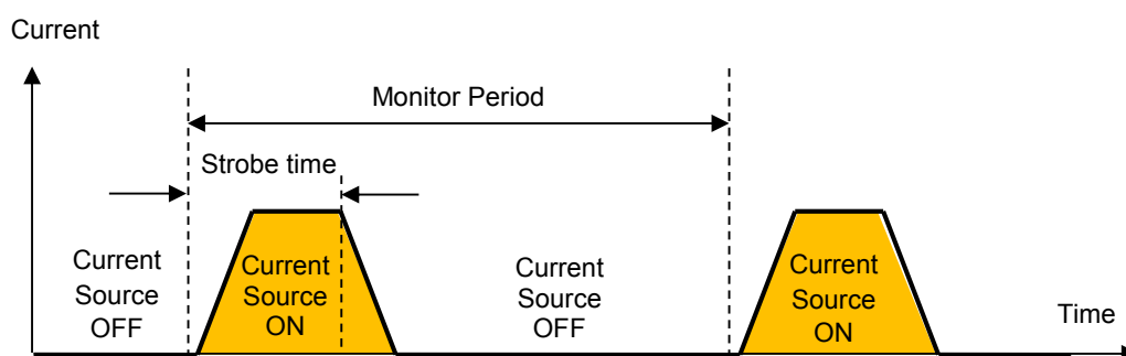
Figure 13. Intermittent Monitoring
