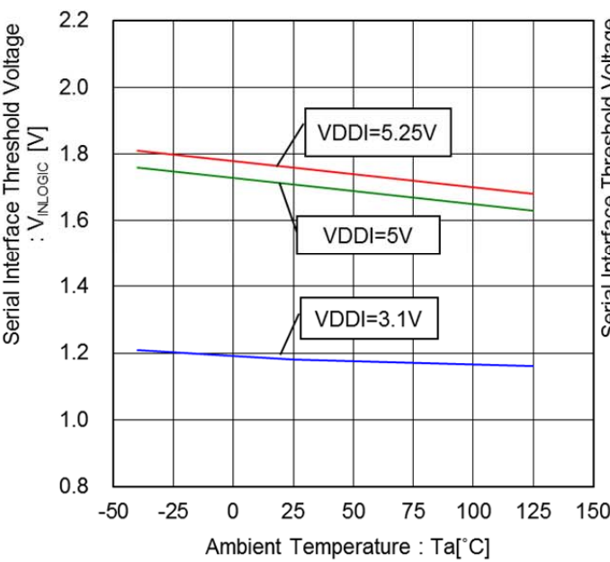
Figure 79. Serial Interface Threshold Voltage vs Ambient Temperature
