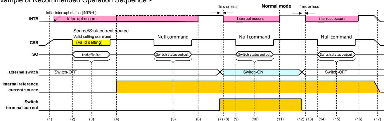
Figure 7. Basic Operation 1
