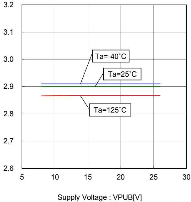
Figure 74. High to Low Switch Detection Threshold Voltage (3.0V Setting) vs Supply Voltage
