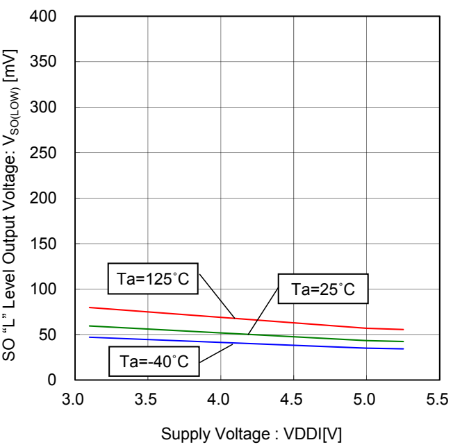
Figure 92. SO "L" Level Output Voltage vs Supply Voltage ( I_{SINK}=1.6mA )
