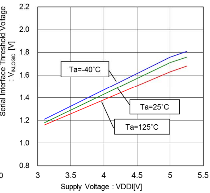
Figure 80. Serial Interface Threshold Voltage vs Supply Voltage
