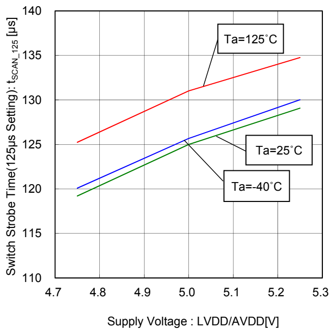
Figure 112. Switch Strobe Time(125µs Setting) vs Supply Voltage
