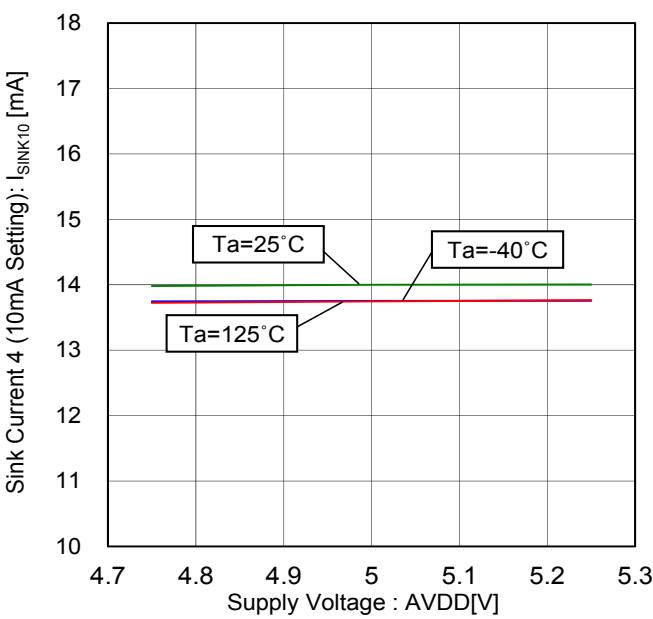
Figure 60. Sink Current 4 (10mA Setting) vs Supply Voltage (8V External Supply)
