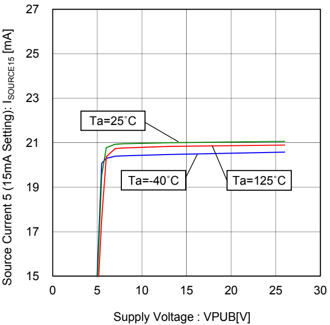
Figure 64. Source Current 5 (15mA Setting) vs Supply Voltage (0V External Supply)
