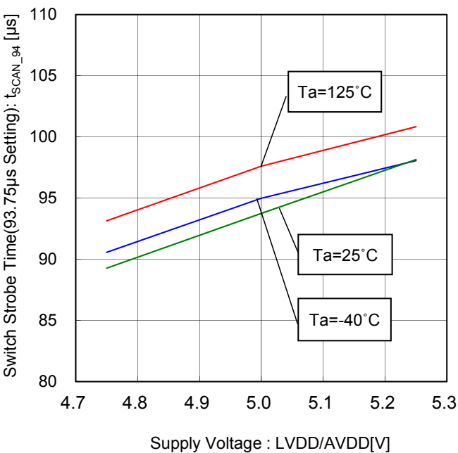
Figure 110. Switch Strobe Time(93.75µs Setting) vs Supply Voltage
