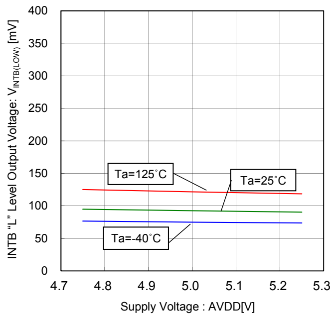
Figure 104. INTB "L" Level Output Voltage vs Supply Voltage ( I_{SINK}=1.0mA )
