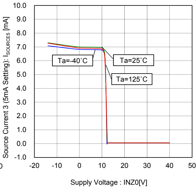
Figure 50. Source Current 3 (5mA Setting) vs Supply Voltage
