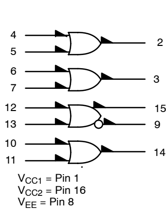
Figure 1. Logic Diagram
