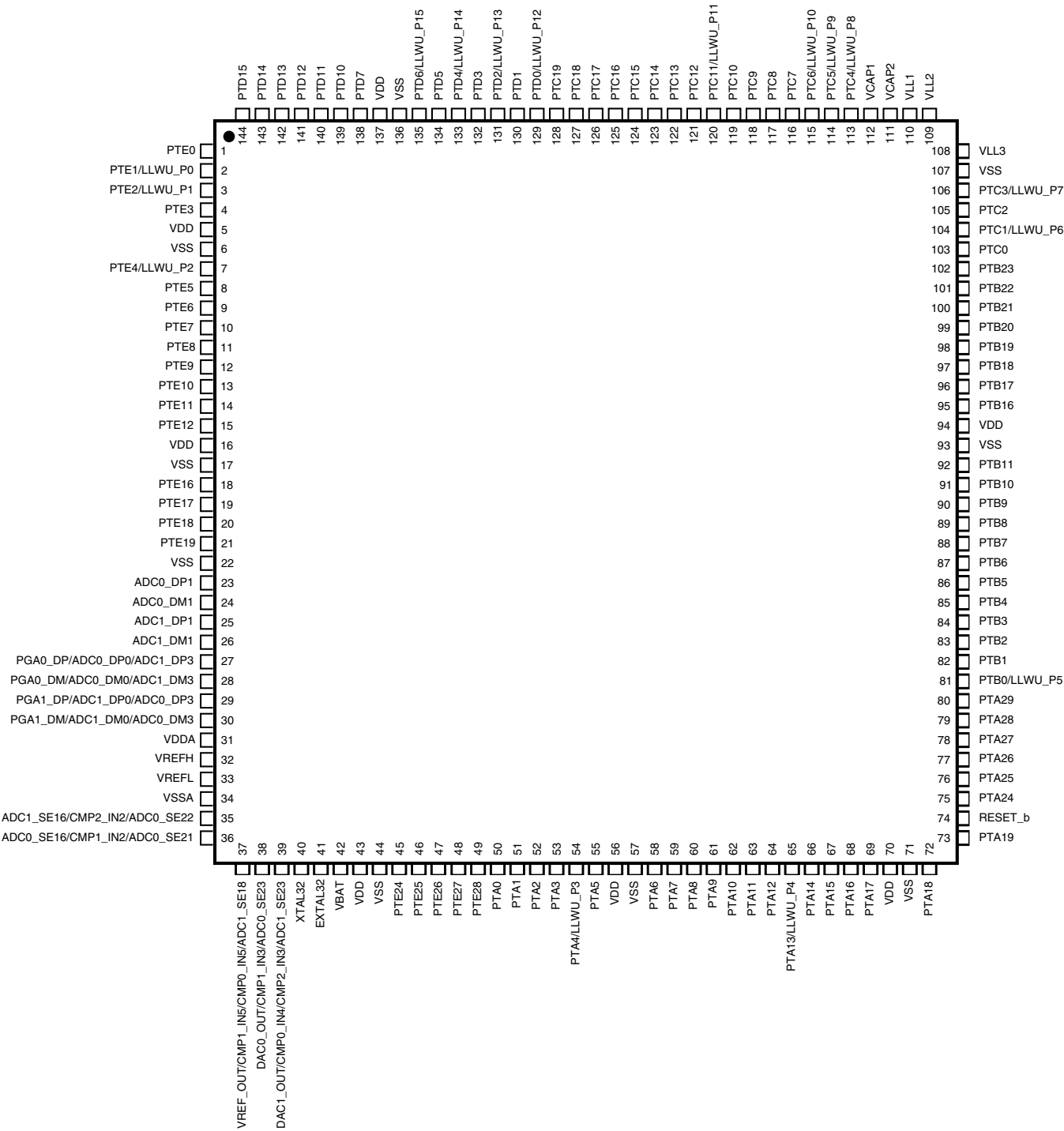
Figure 32. K30 144 LQFP Pinout Diagram
