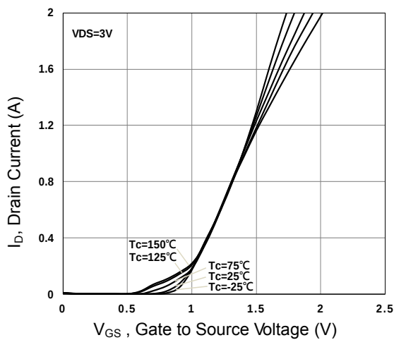
Figure 9. Transfer Characteristics
