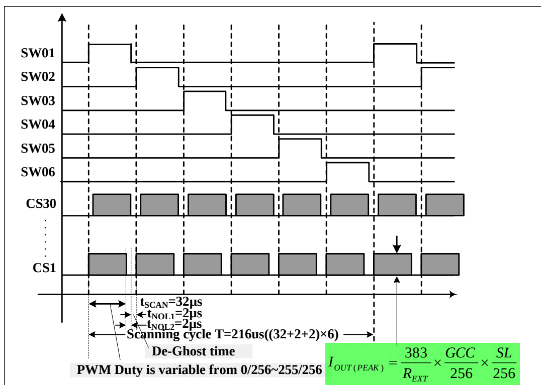
Figure 12 Scanning Timing
