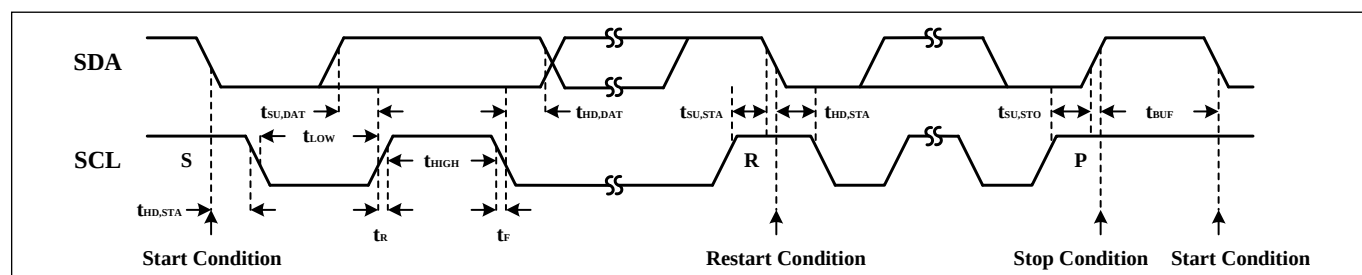
Figure 4 Interface Timing
