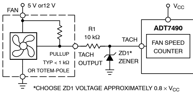
Figure 44. Fan with Strong TACH. Pullup to > V_{CC} or Totem-Pole Output, Clamped with Zener Diode and Resistor
