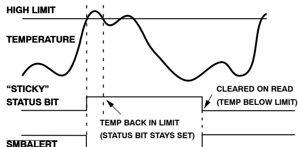
Figure 30. \overline{\text{SMBALERT}} and Status Bit Behavior
