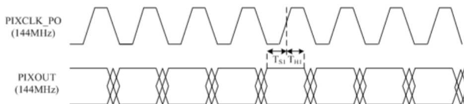
Figure 7-1 OTDM is operated at 144MHz
