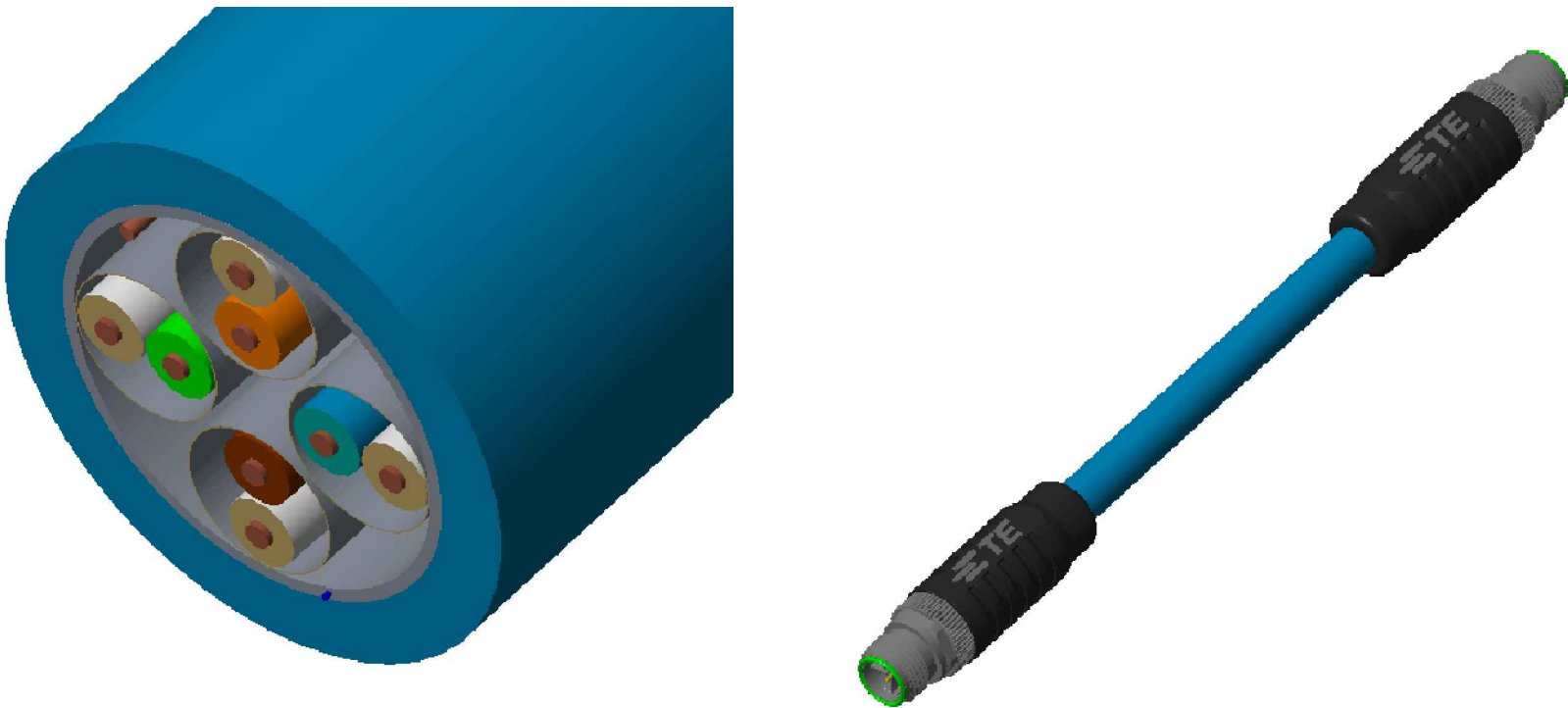
SECTIONAL ISO VIEW OF THE CABLE
