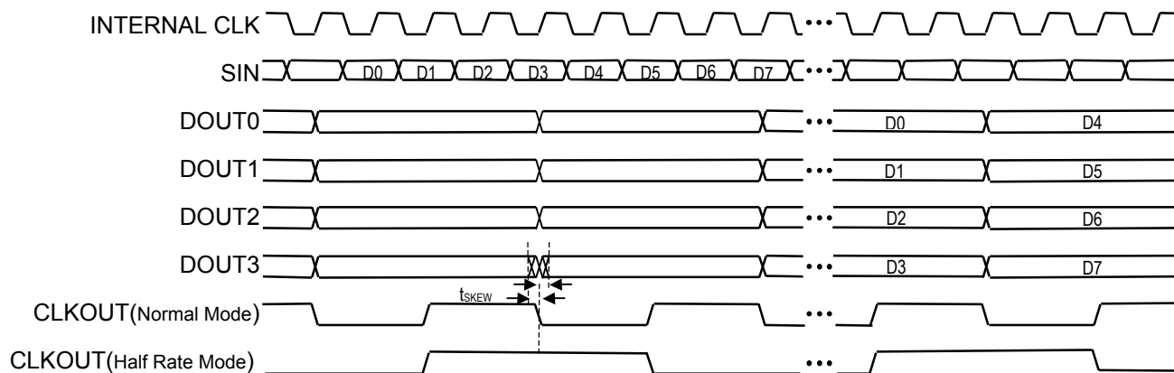
Figure 1. 1:4 Serial-to-Parallel Conversion
