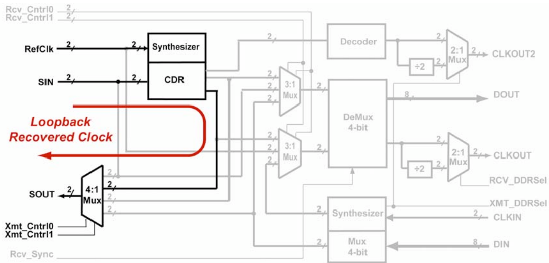
Figure 7. Remote Loopback Recovered Clock Flow
