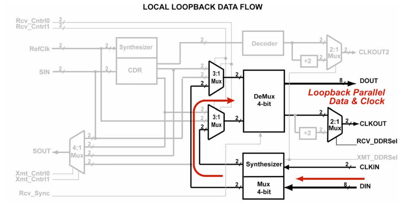
Figure 10. Local Loopback Data Flow
