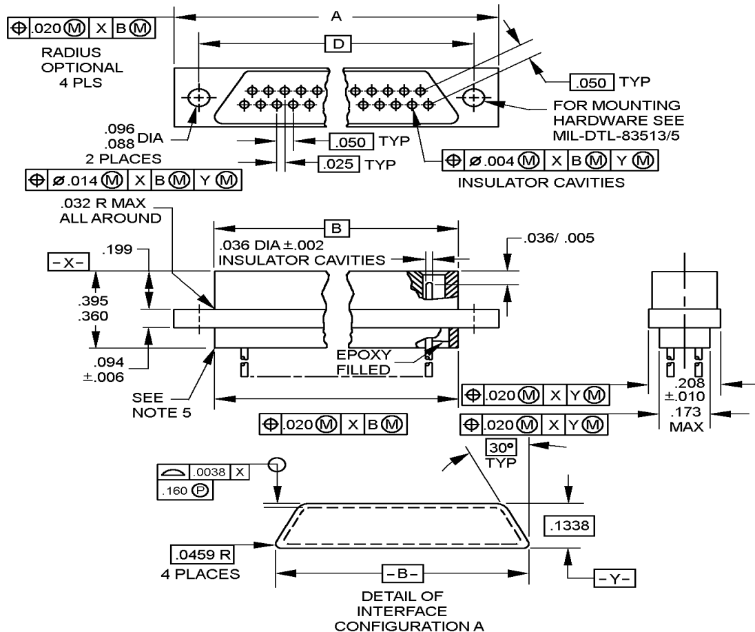
FIGURE 1. Connector, plug, .050 spacing.
