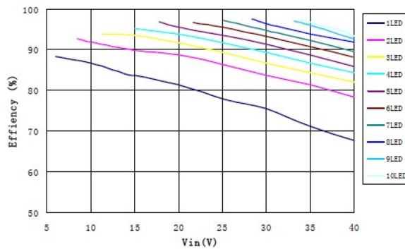
Efficiency vs. No. of LEDs L=47\mu\text{H} , R_s=0.33\Omega
