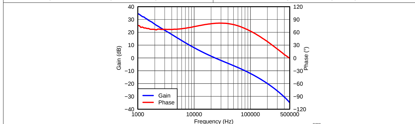
Figure 10. VOUT = 1.8 V, IOUT = 4 A, COUT1 = 47 µF ceramic, COUT2 = 100 µF POSCAP, fSW = 1 MHz
