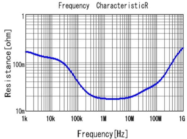
■ ECASD40J106M055K00 R DC0V, 25degC
