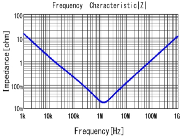
■ ECASD40J106M055K00 |Z| DC0V, 25degC
