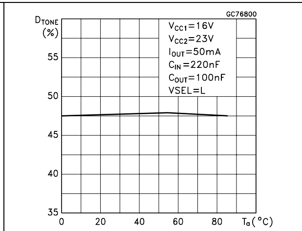
Figure 4. Tone duty cycle vs temperature
