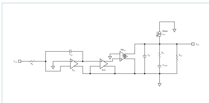
Figure 62 — LGH amplifier small-signal model
