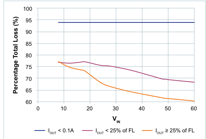
Figure 46 — V_{OUT} = 18V
