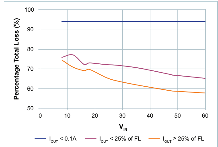
Figure 47 — V_{OUT} = 24V
