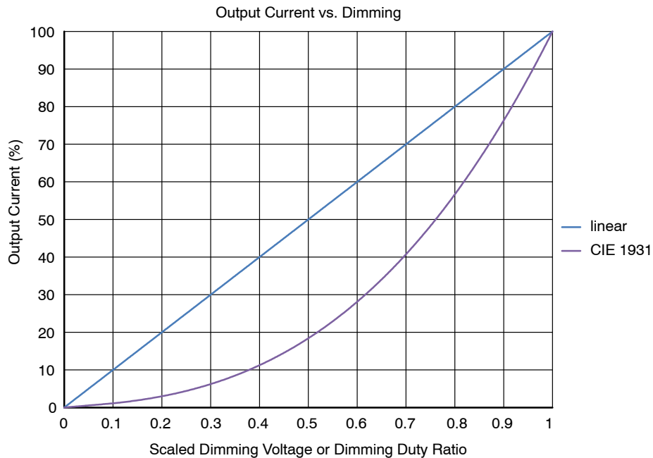
Figure 67. Dimming Curves
