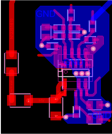
Figure 63. PCB Layout Example
