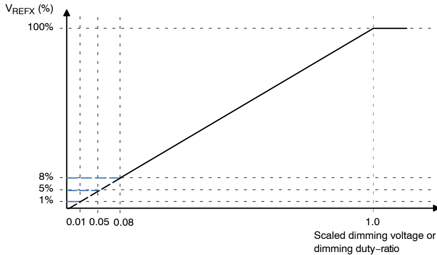
Figure 66. Dimming Clamp Options
