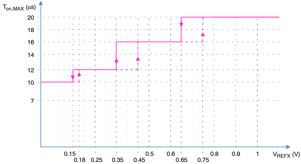
Figure 72. Variable Maximum On-time, 20-μs Option
