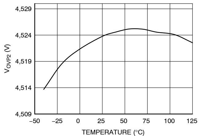
Figure 44. V OVP2 vs. Temperature
