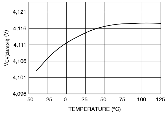
Figure 42. V CV(clampH) vs. Temperature
