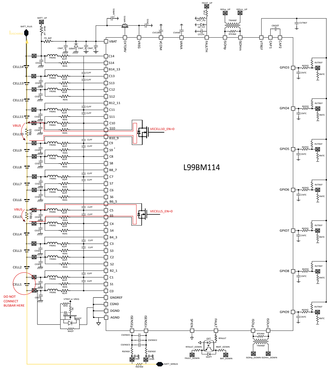
Figure 42. How to connect cell modules and busbar
