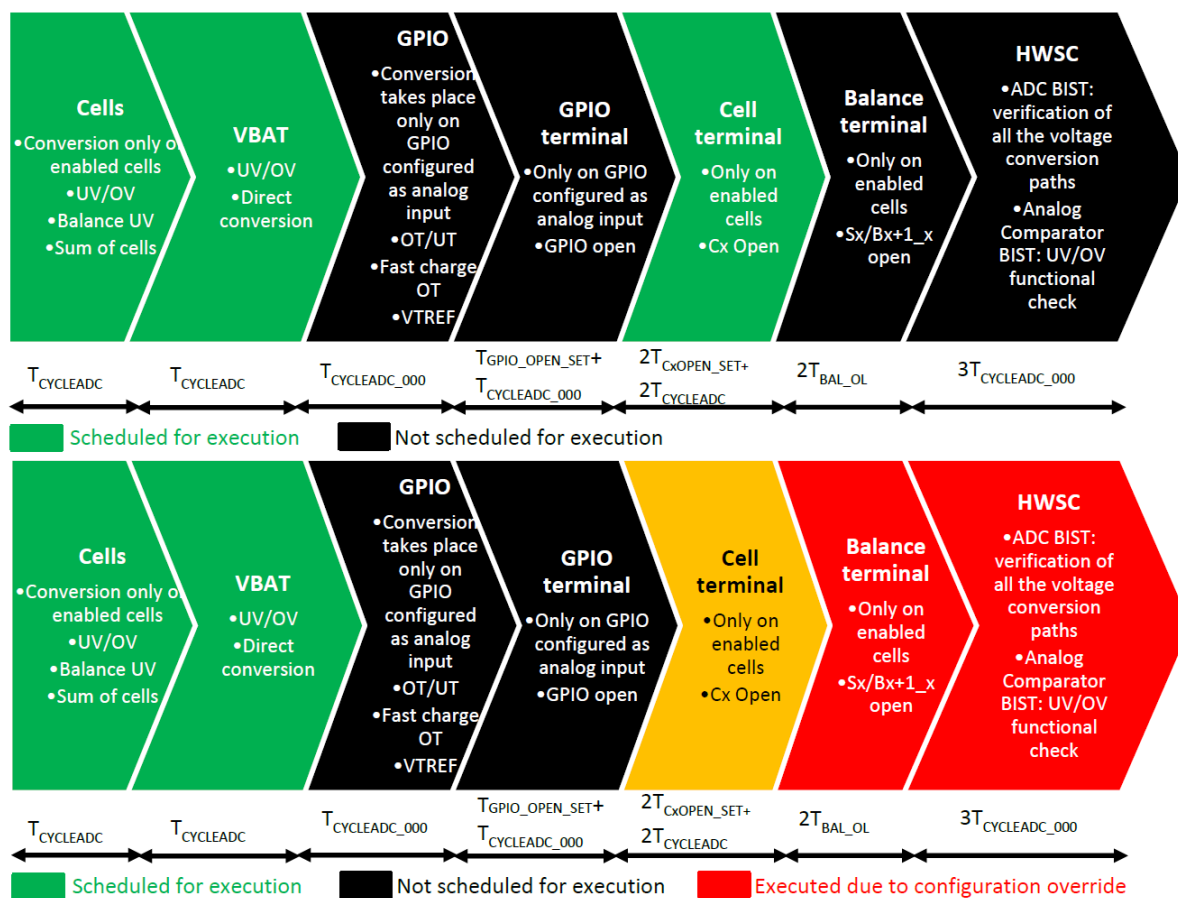
Figure 26. Example of configuration override: a failure detected during Cell Terminal diagnostics (yellow background) causes the following two steps (red background) to be executed
