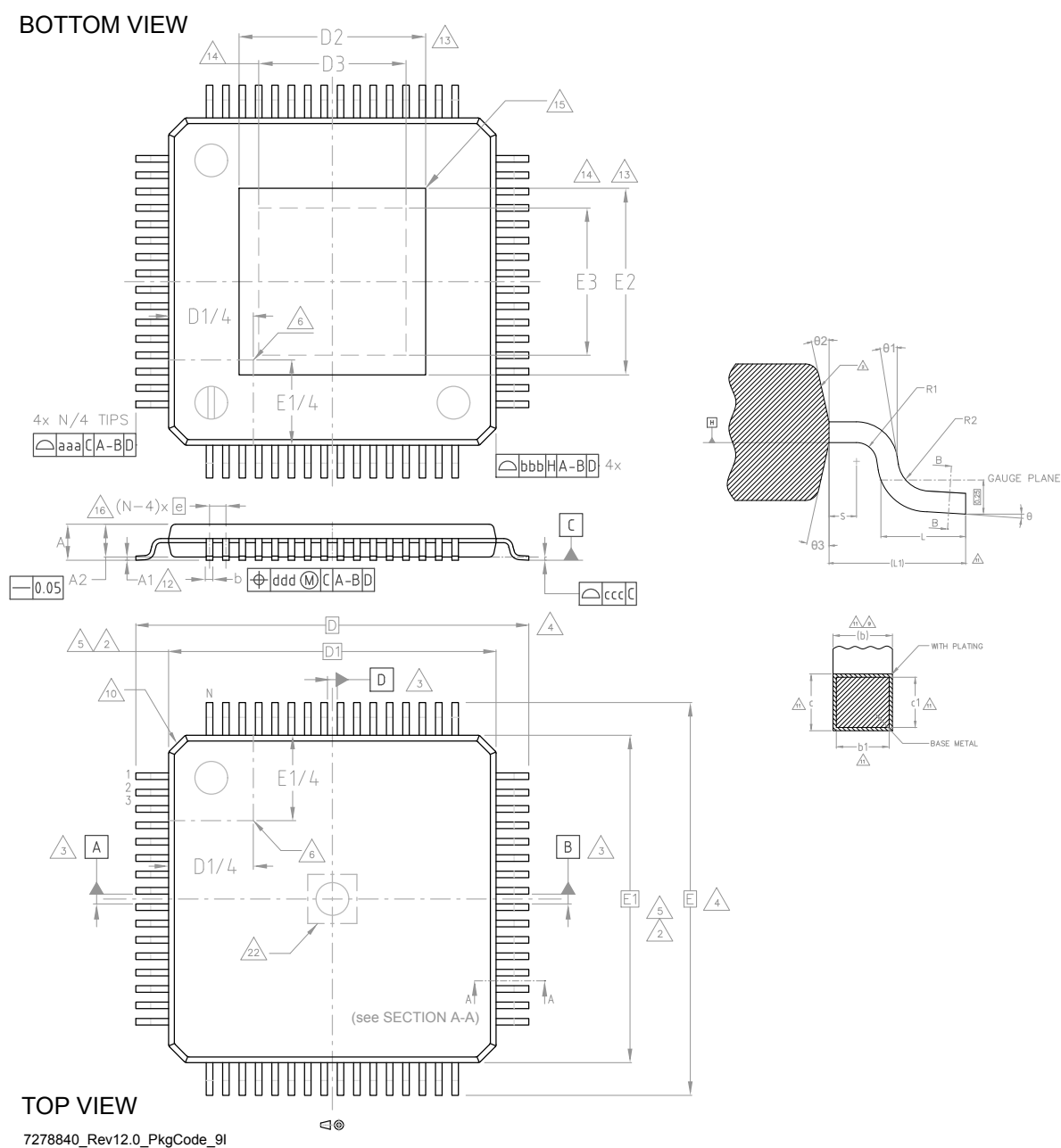
Figure 44. TQFP 10x10 64L exposed pad down package outline
