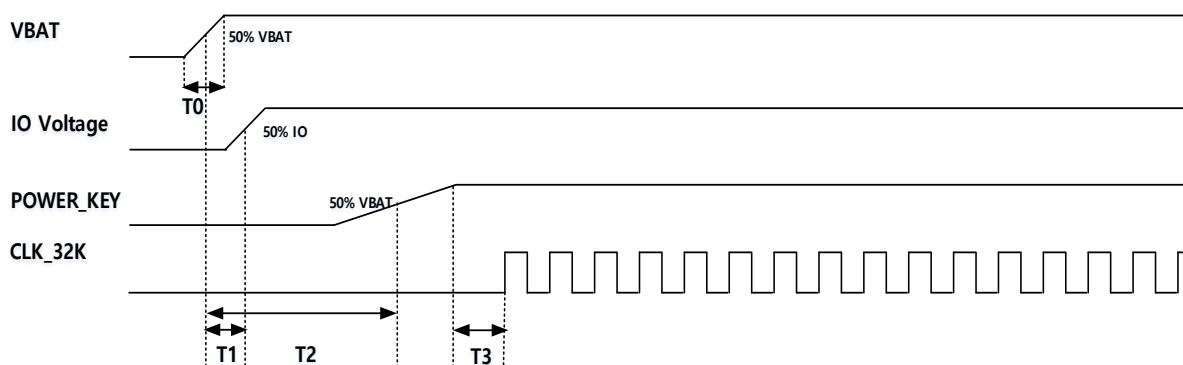
Figure 6. Power-on sequence
