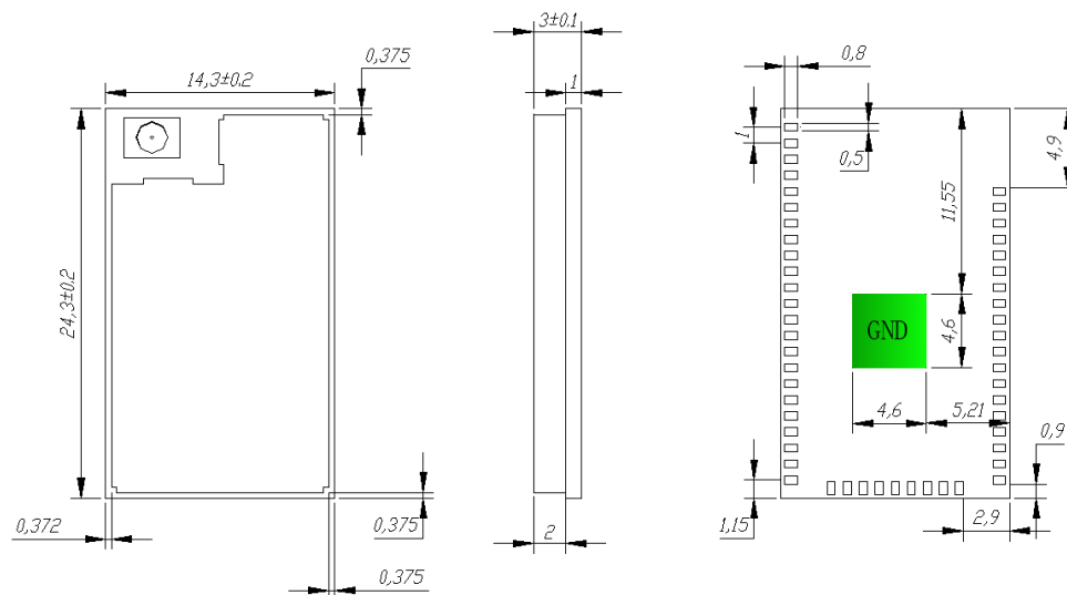
Figure 9. AAE module dimension
