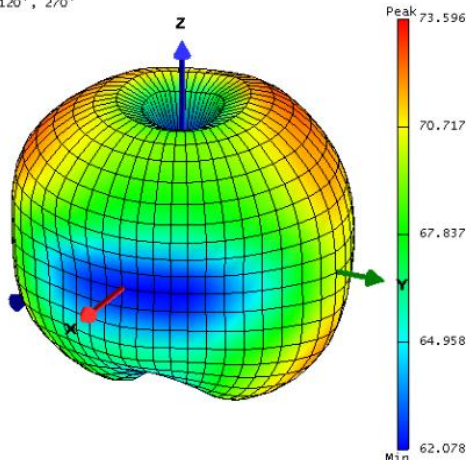
Figure 4. TIS 3D
