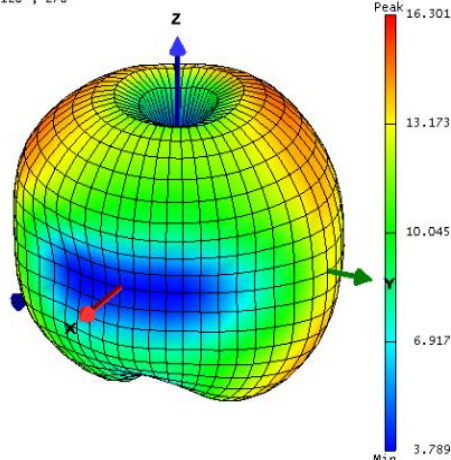
Figure 5. TRP 3D
