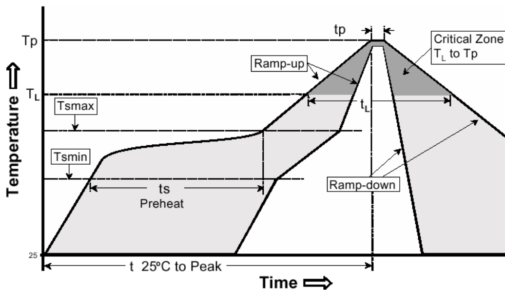
Figure 14. Reflow condition
