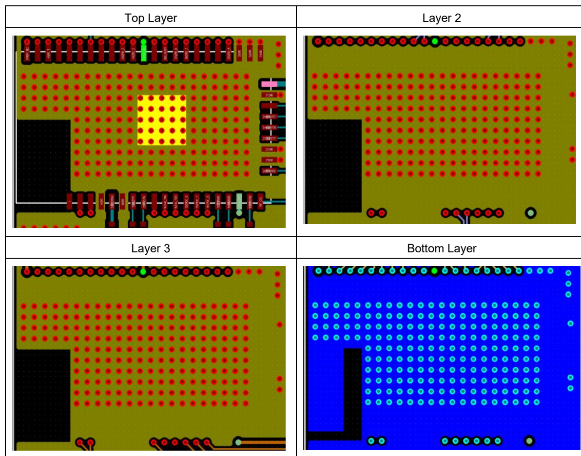
Figure 13. 4-layer PCB example
