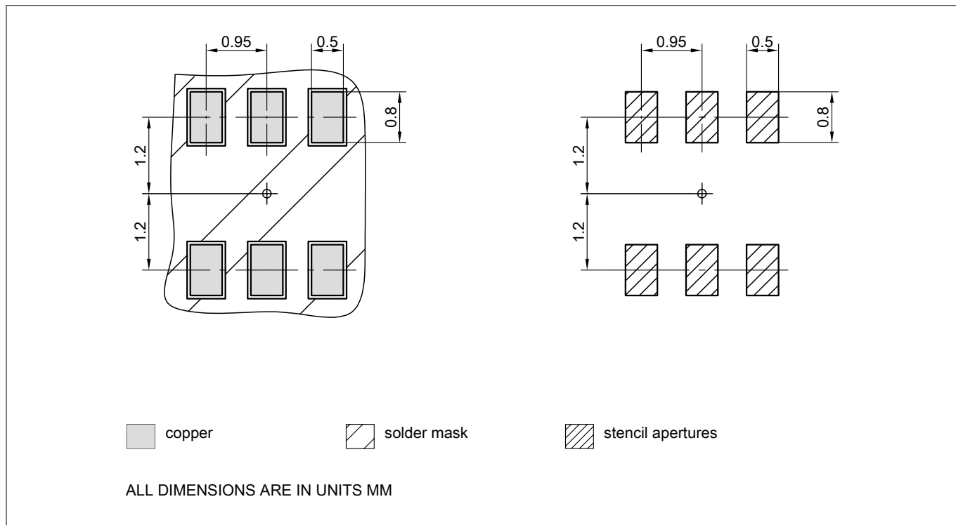
Figure 16 PG-SOT23-6 footprint
