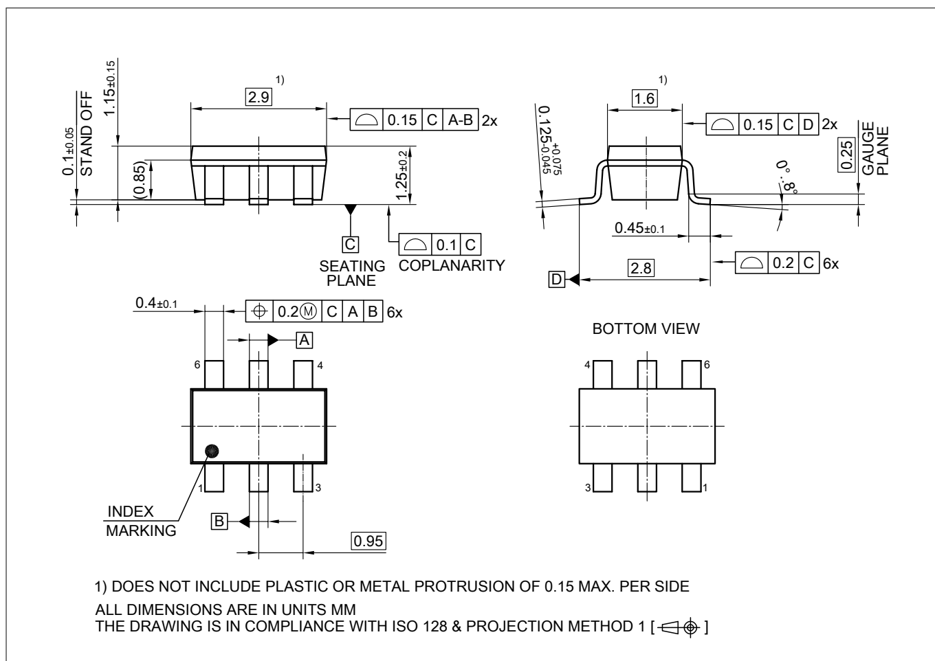
Figure 15 PG-SOT23-6 outline
