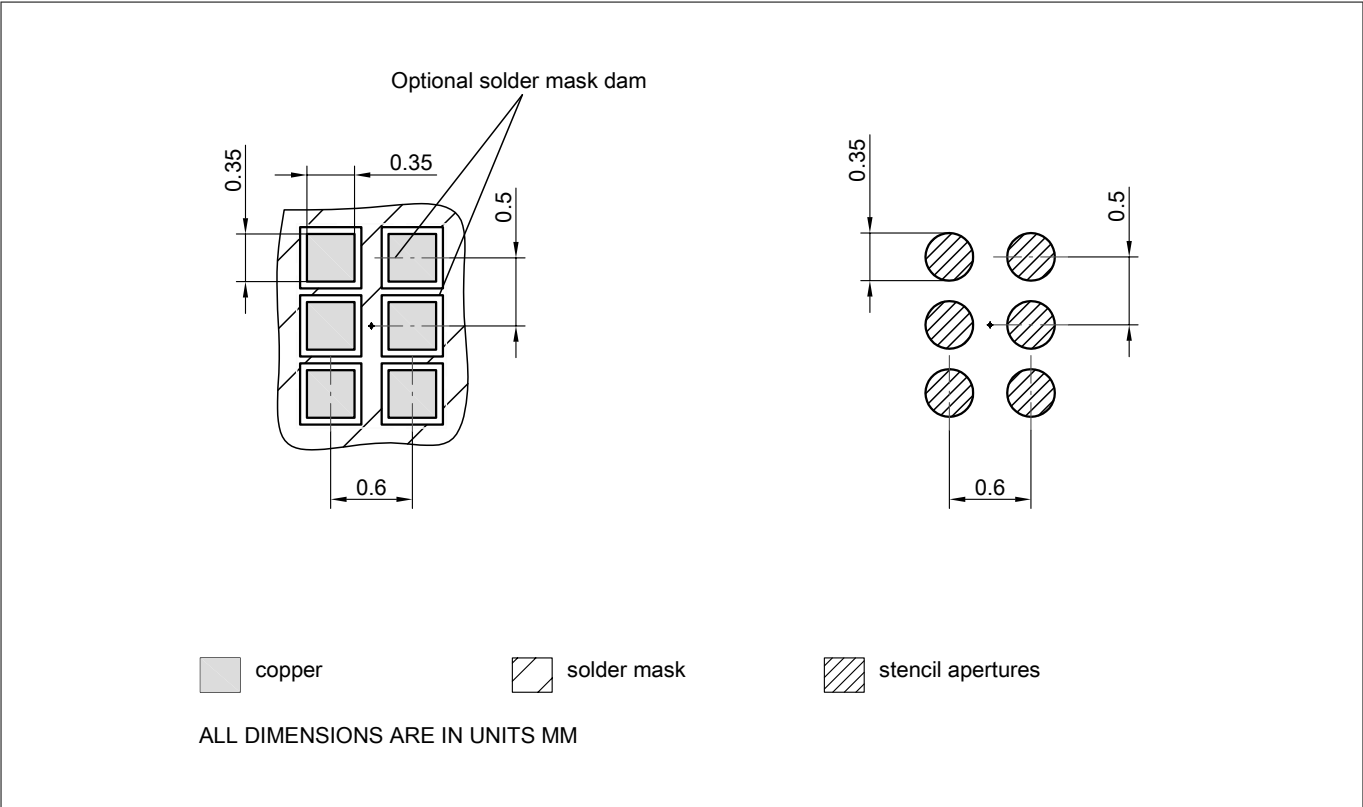
Figure 20 PG-TSNP-6 footprint
