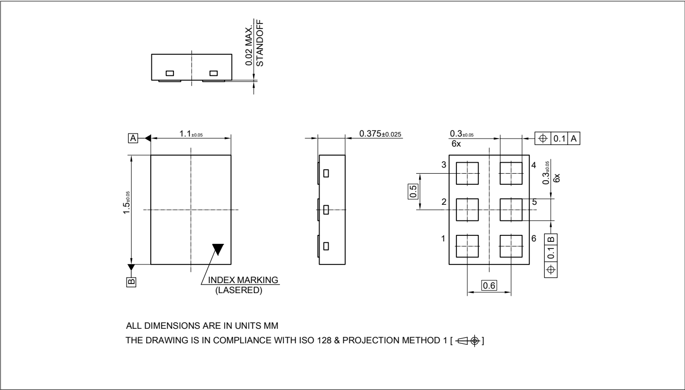
Figure 19 PG-TSNP-6 outline
