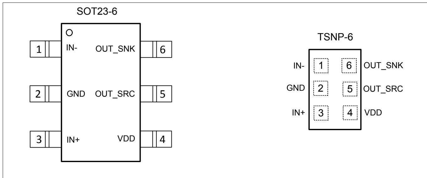
Figure 2 Pin configuration SOT23-6 and TSNP-6 6-pin packages (top view)
