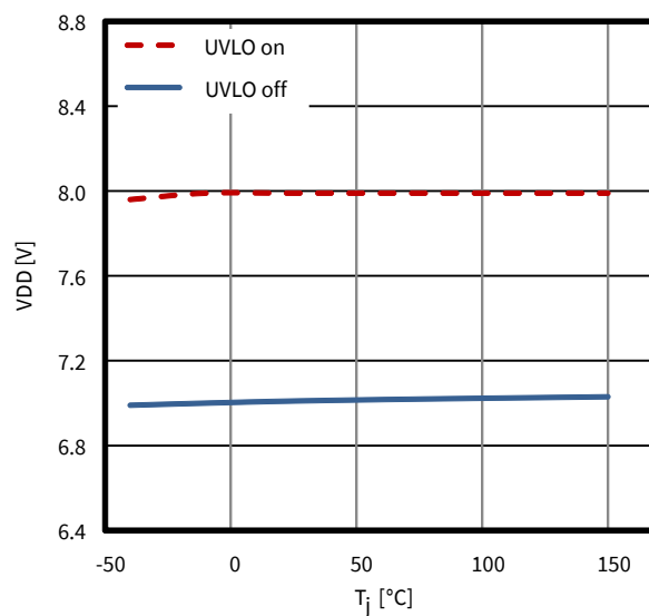
4. Undervoltage lockout threshold (1EDN9550) vs temperature
