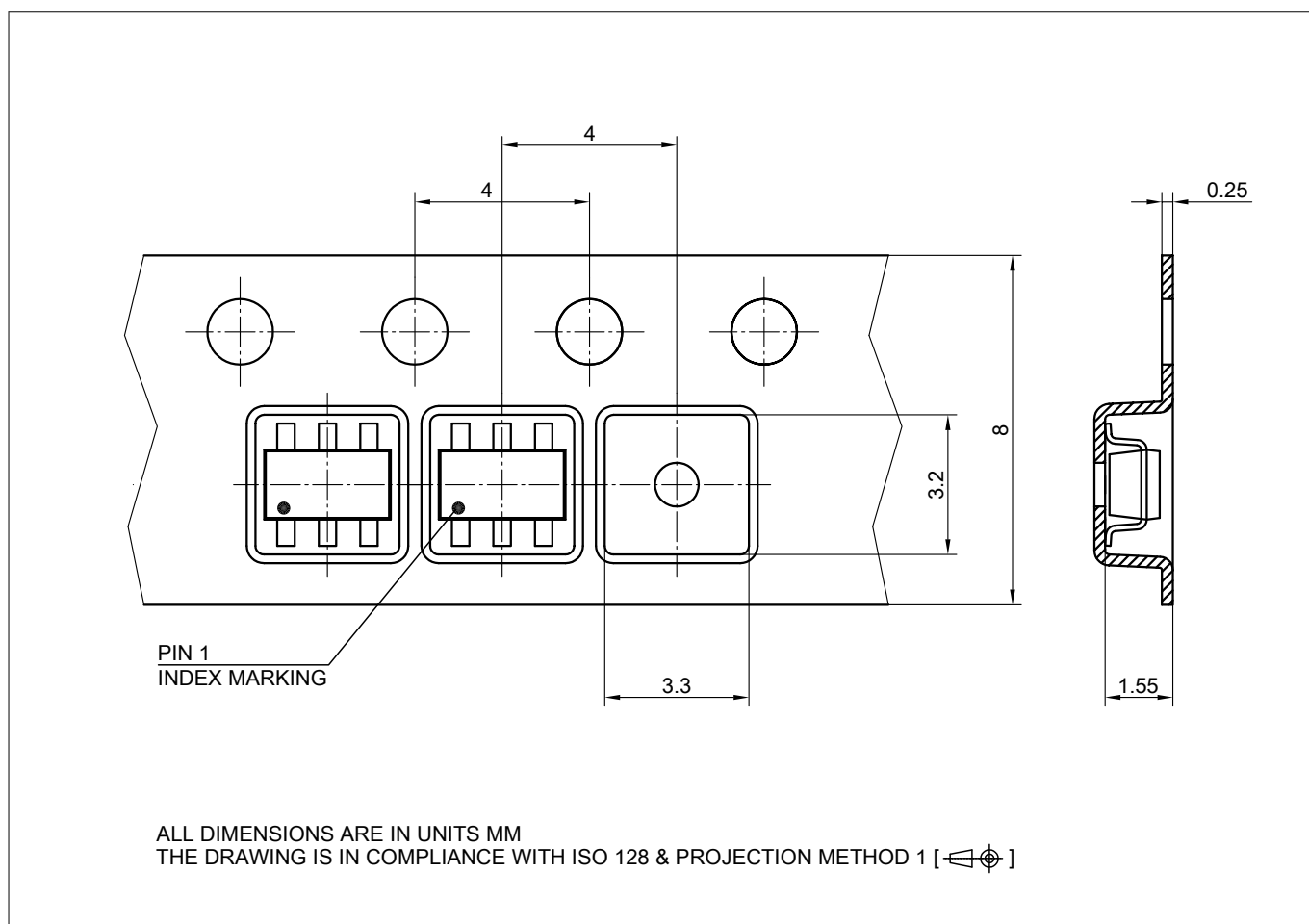
Figure 17 PG-SOT23-6 packaging
