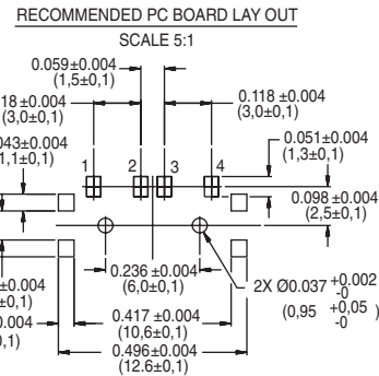
JSM08022SAQNL SPDT Surface Mount Momentary only
