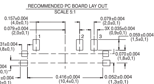
JSM05000SAQN SP3T Surface Mount Momentary both sides
