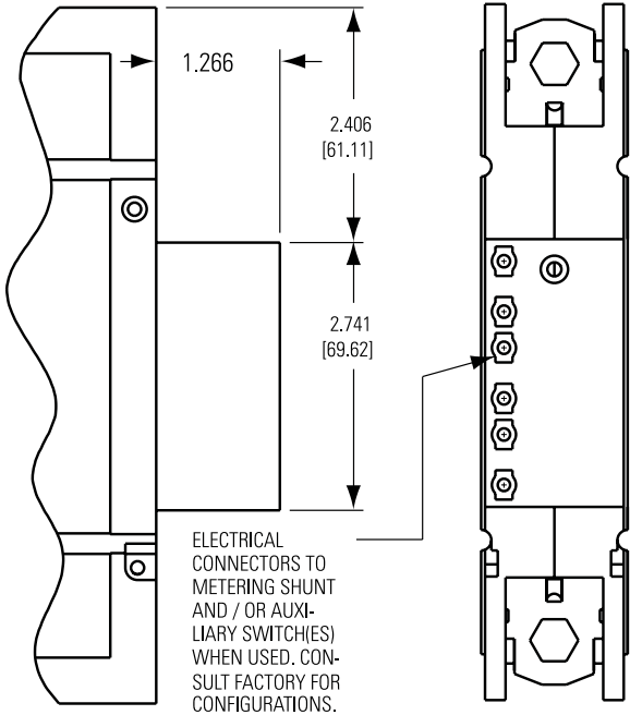
Metering Shunt
