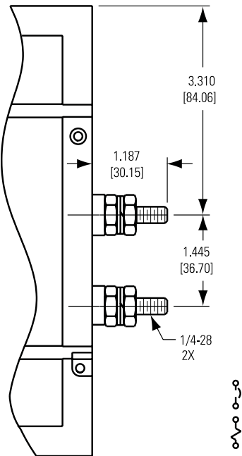
Relay Trip
