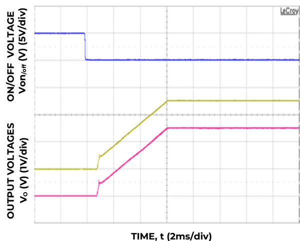
Figure 23. Typical Start-up Using On/Off Voltage ( V_{in} = 12\text{V} , I_o = I_{o1,max}, I_{o2,max} ).
