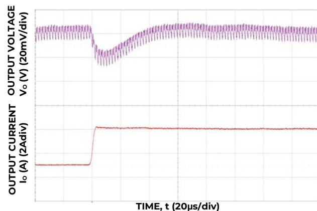
Figure 10. Transient Response to Dynamic Load Change on one output from 50% to 100% on at 12V IN , C_{OUT} = 3 \times 4.7\mu\text{F} + 2 \times 330\mu\text{F} , C_{TUNE} = 2700\text{pF} , R_{TUNE} = 300\Omega
