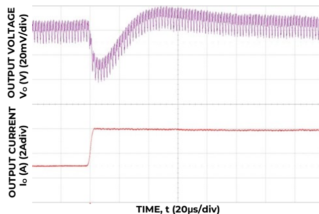
Figure 16. Transient Response to Dynamic Load Change on one output from 50% to 100% on at 12V in , C_{out} = 3 \times 47\mu\text{F} + 1 \times 330\mu\text{F} , C_{Tune} = 1800\text{pF} , R_{Tune} = 300\Omega
