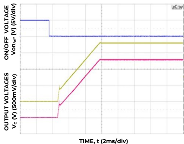
Figure 17. Typical Start-up Using On/Off Voltage ( V_{IN} = 12\text{V} , I_o = I_{o1,max}, I_{o2,max} ).
