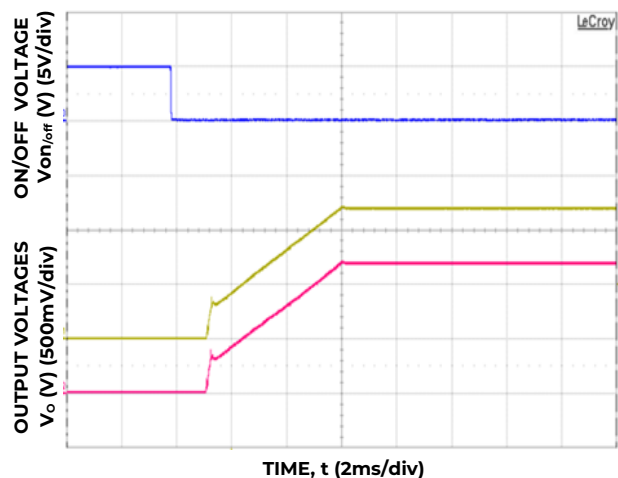
Figure 11. Typical Start-up Using On/Off Voltage ( V_{IN} = 12\text{V} , I_o = I_{o1,max}, I_{o2,max} ).
