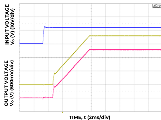
Figure 18. Typical Start-up Using Input Voltage ( V_{IN} = 12\text{V} , I_o = I_{o1,max}, I_{o2,max} ).
