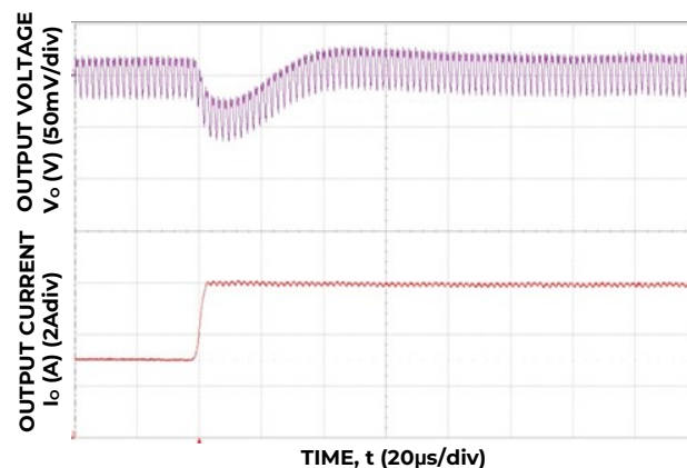
Figure 22. Transient Response to Dynamic Load Change on one output from 50% to 100% on at 12V in , C_{out} = 2 \times 47\mu\text{F} + 1 \times 330\mu\text{F} , C_{Tune} = 1500\text{pF} , R_{Tune} = 300\Omega
