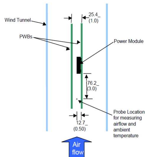
Figure 46. Thermal Test Setup.
