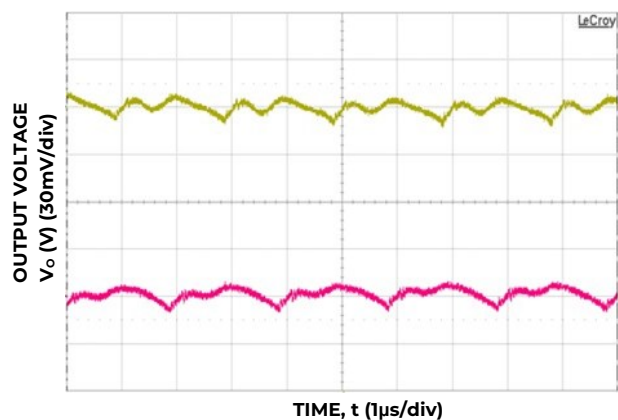
Figure 9. Typical output ripple and noise ( C_O = 2 \times 4.7\text{nF} + 2 \times 47\mu\text{F} ceramic, V_{IN} = 12\text{V} , I_o = I_{o1,max}, I_{o2,max} ).
