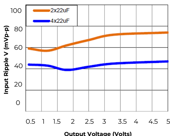
Figure 37. Input ripple voltage for various output voltages with 2x22 μF or 4x22 μF ceramic capacitors at the input (2 x 6A load). Input voltage is 12V. Scope BW: 20MHz
