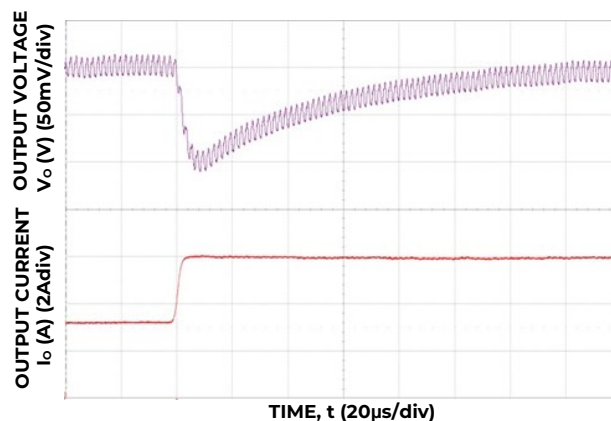
Figure 34. Transient Response to Dynamic Load Change on one output from 50% to 100% on at 12V in , C_{out} = 4 \times 47\mu F , C_{Tune} = 470pF , R_{Tune} = 300\Omega
