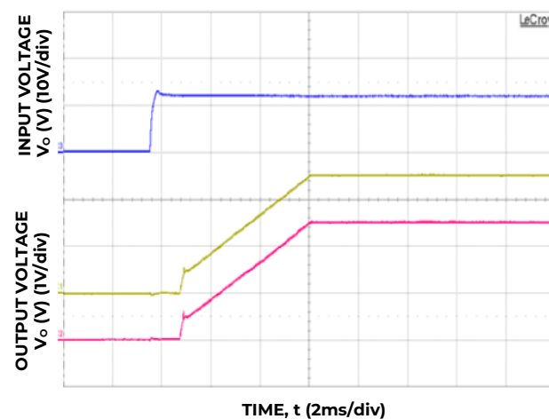
Figure 24. Typical Start-up Using Input Voltage ( V_{in} = 12\text{V} , I_o = I_{o1,max}, I_{o2,max} ).
