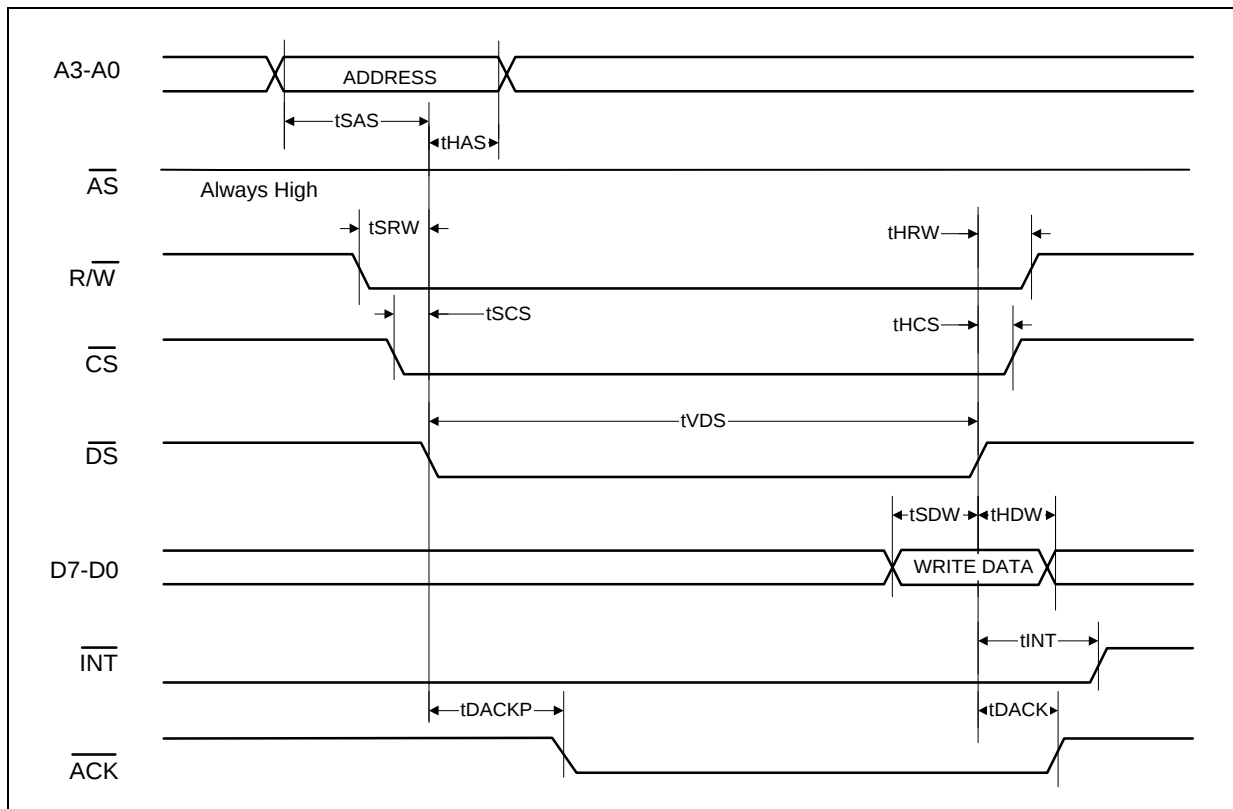
Figure 26. Non-Multiplexed Motorola Mode Write Timing
