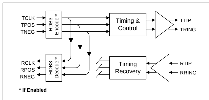
Figure 8. Digital Loopback
