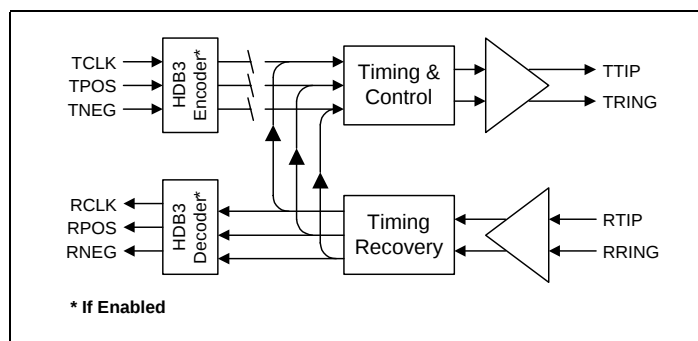
Figure 9. Remote Loopback
