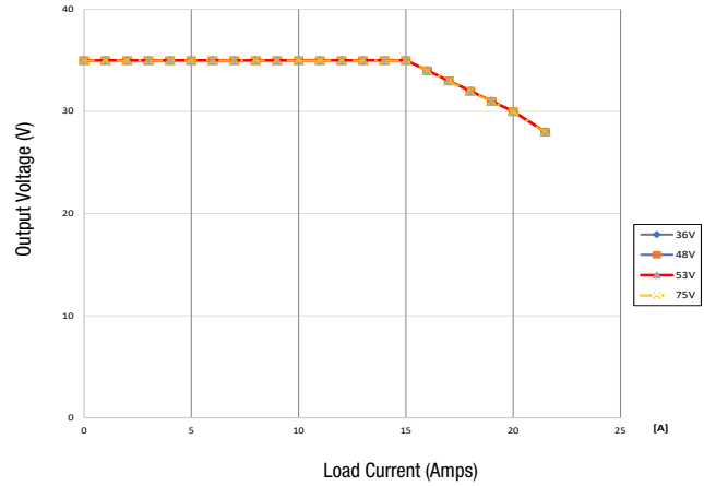
Output Voltage vs. Load Current @ 25°C
