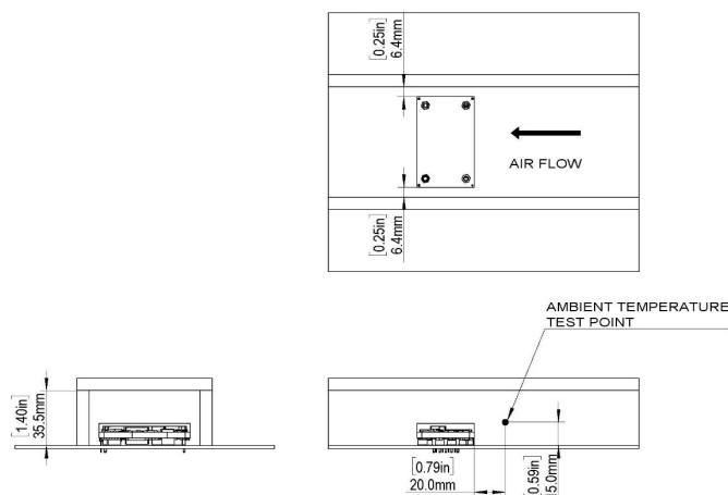
Wind Tunnel Test Set-up
