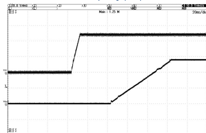
Start-up Voltage (48Vin)
