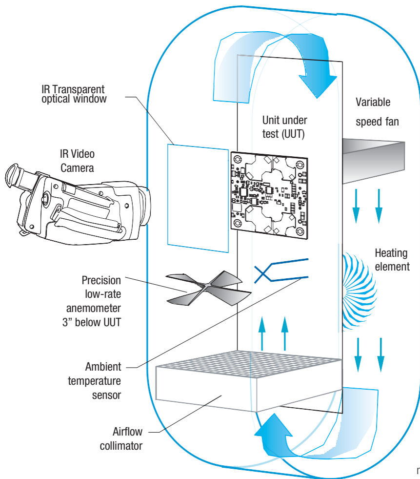
Vertical Wind Tunnel
