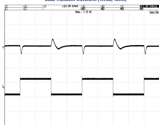
Load Transient Waveform (1A/uS, 48Vin)
