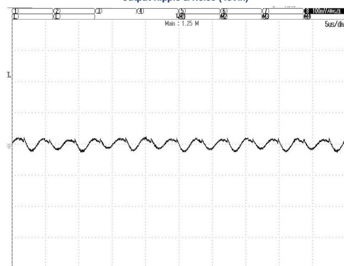
Output Ripple & Noise (48Vin)
