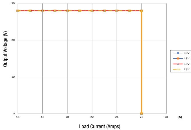
Current Limit Characteristics @ 25°C
