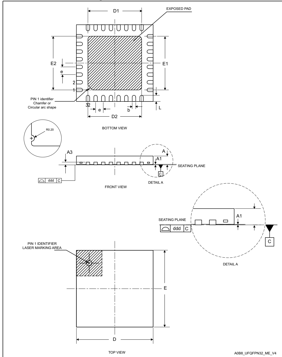
Figure 41. UFQFPN32 - Outline
