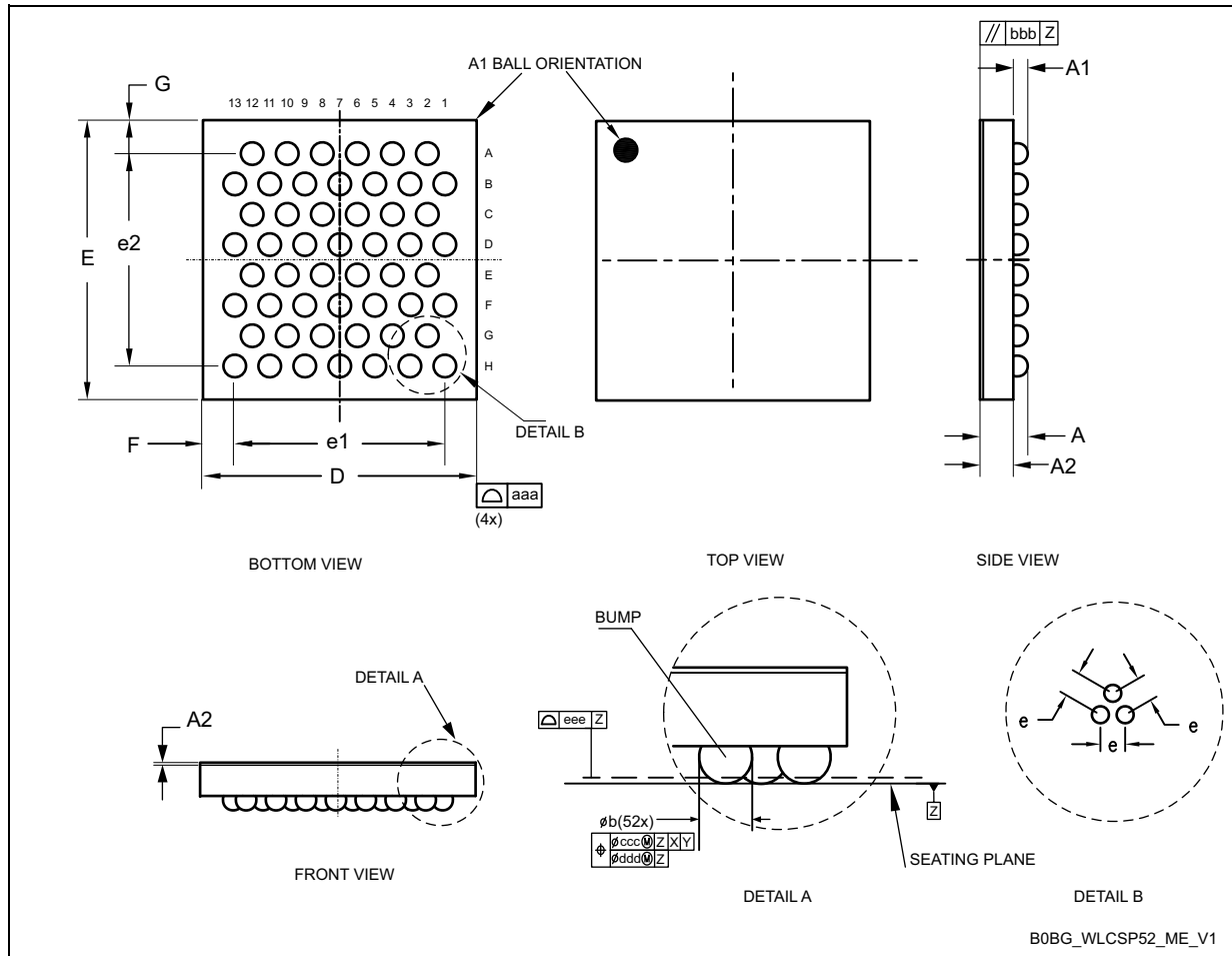
Figure 47. WLCSP52 - Outline
