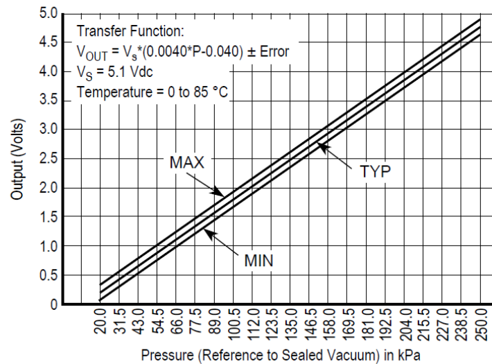
Figure 6. Transfer function
