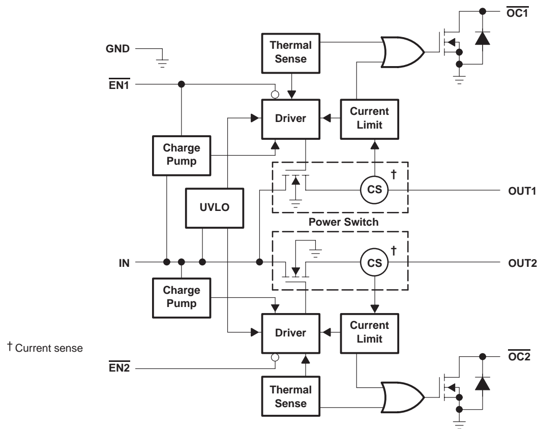
TPS2042 functional block diagram
