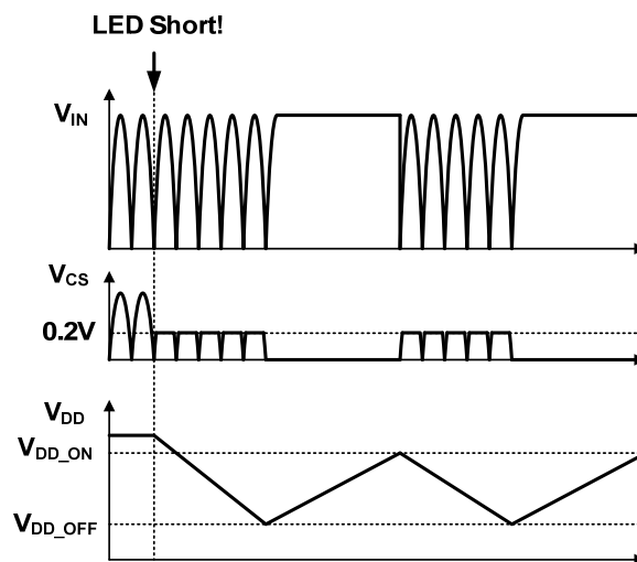
Figure 23. Waveforms in Short-LED Condition
