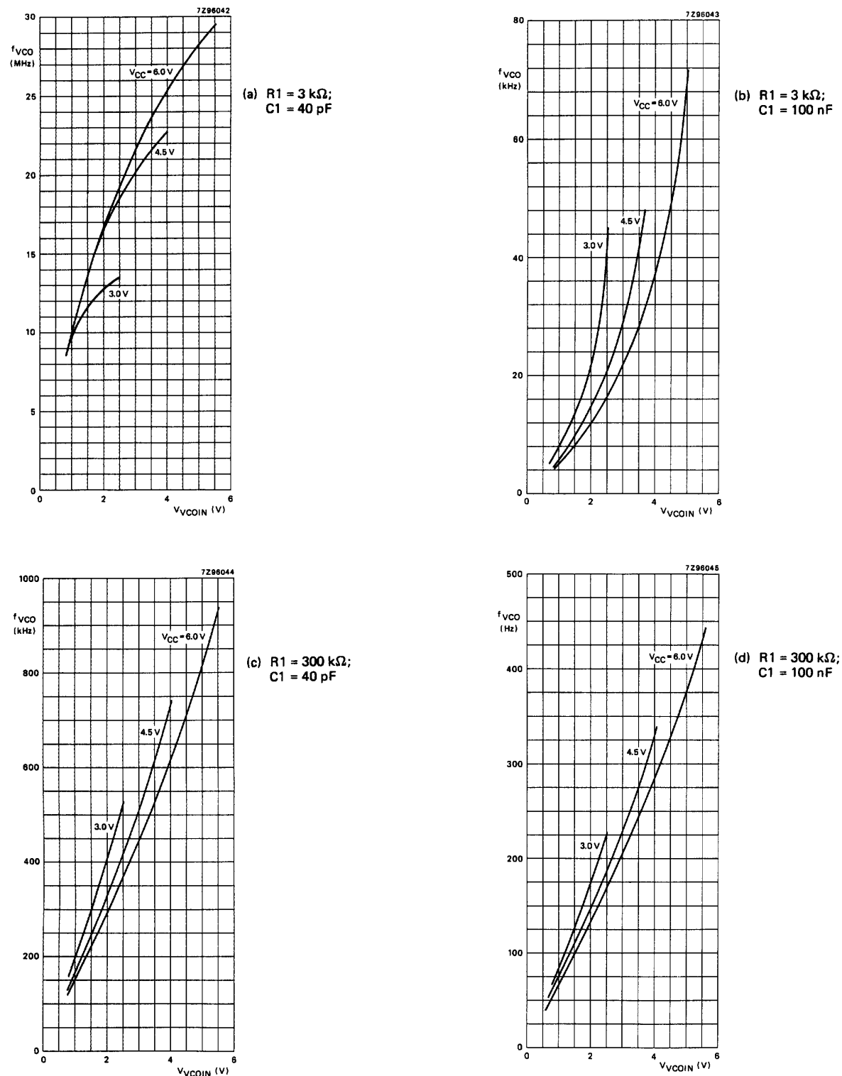
Fig.17 Graphs showing VCO frequency ( f_{VCO} ) as a function of the VCO input voltage ( V_{VCOIN} ).
