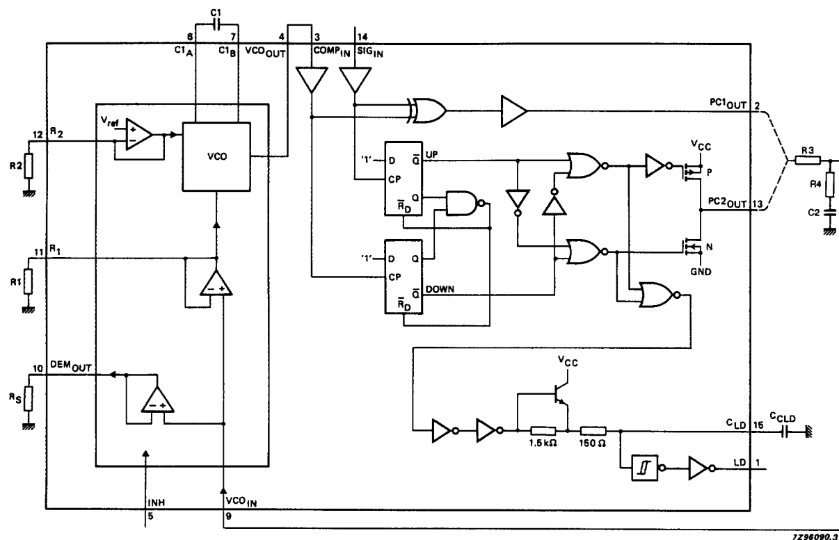
Fig.5 Logic diagram.
