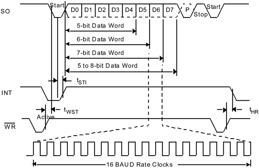
Figure 26. Transmitter Timing
