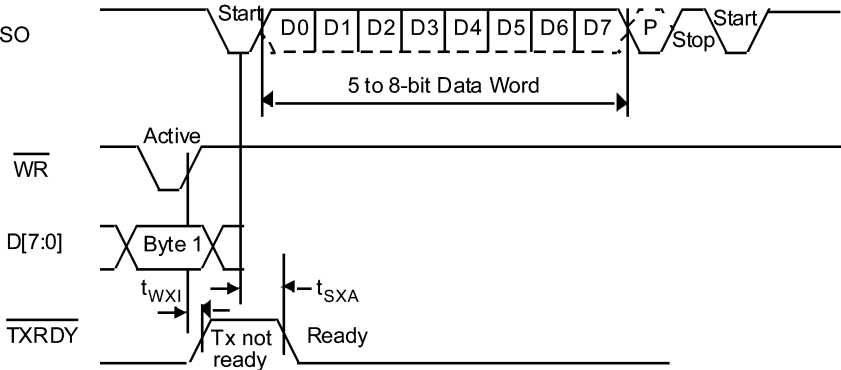
Figure 27. Transmitter Timing Non-FIFO Mode
