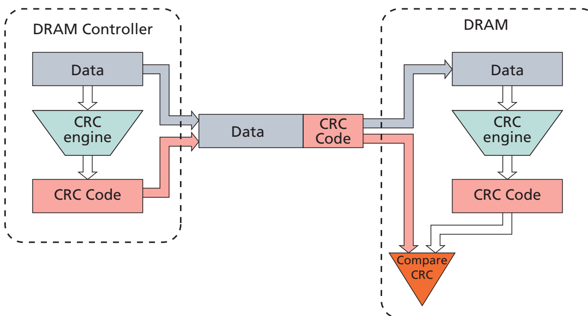
Figure 101: CRC Write Data Operation
