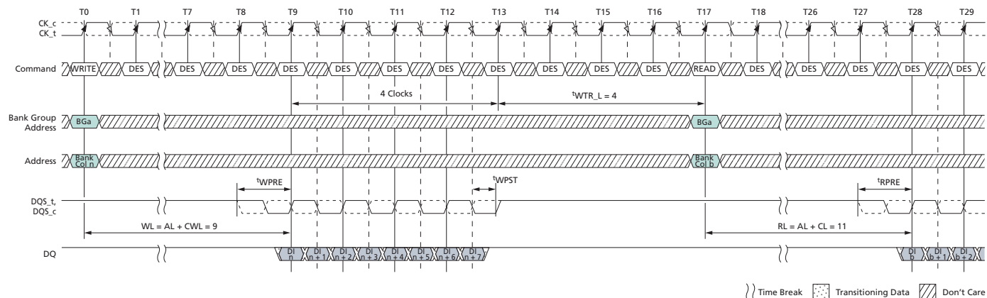
Figure 178: WRITE (BL8) to READ (BL8) with 1^t\text{CK} Preamble in Same Bank Group
