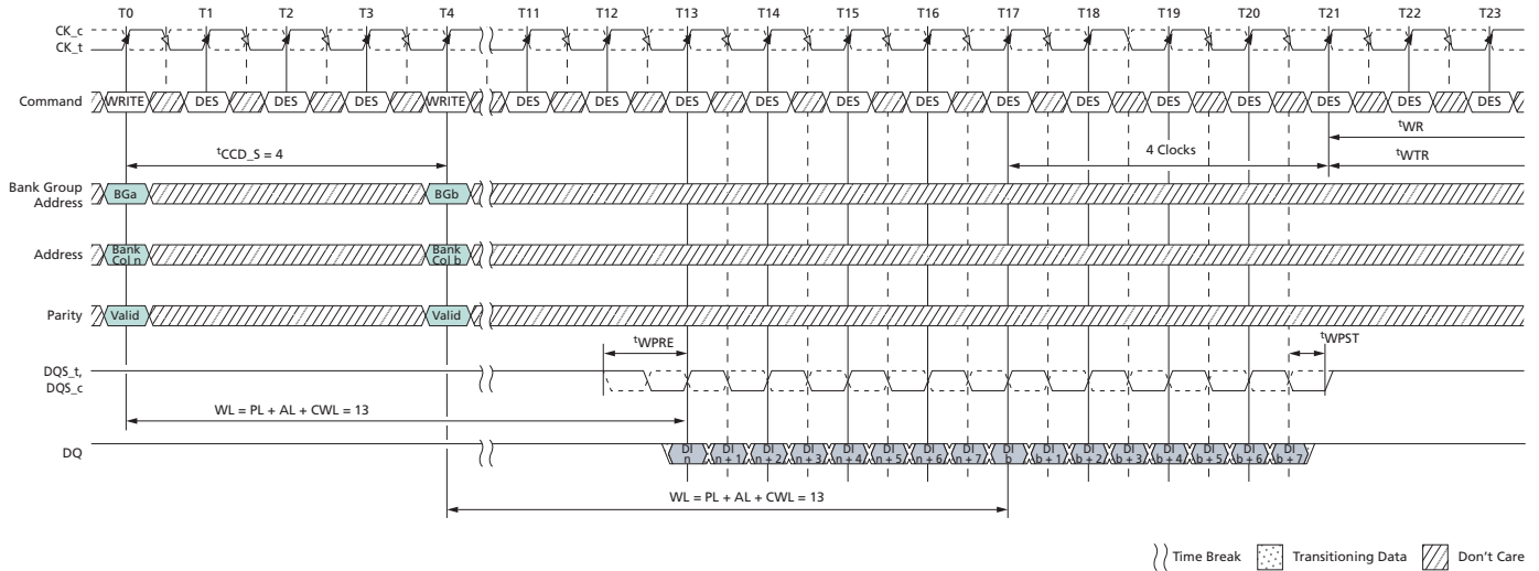
Figure 189: Consecutive Write (BL8) with 1 st CK Preamble and CA Parity in Different Bank Group
