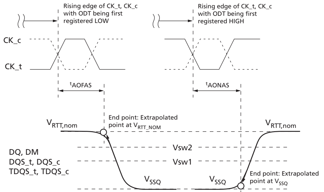
Figure 237: t_{\text{AOFAS}} and t_{\text{AONAS}} Definitions
