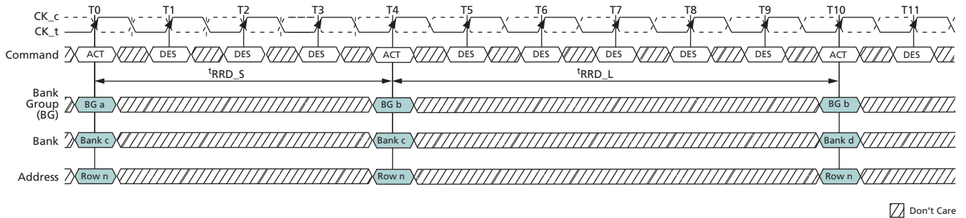
Figure 115: t_{RRD} Timing
