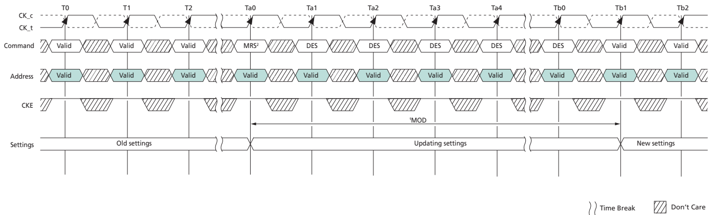
Figure 12: t_{MOD} Timing
