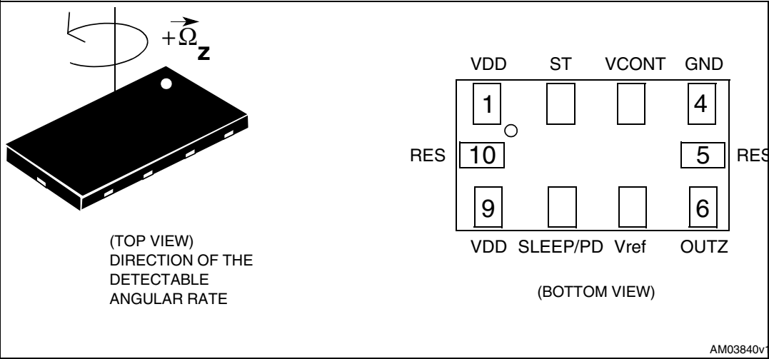
Figure 2. Pin connection
