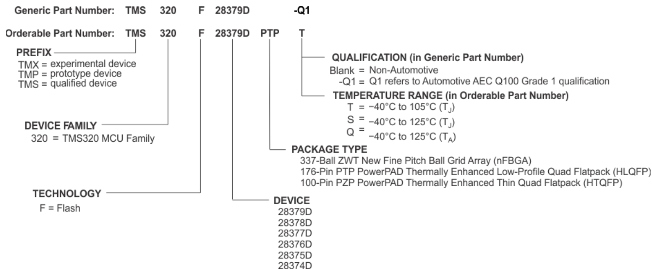
Figure 11-1. Device Nomenclature
