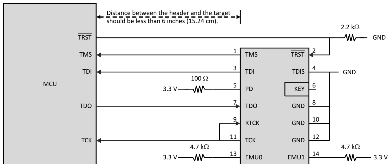
Figure 8-9. Connecting to the 14-Pin JTAG Header
