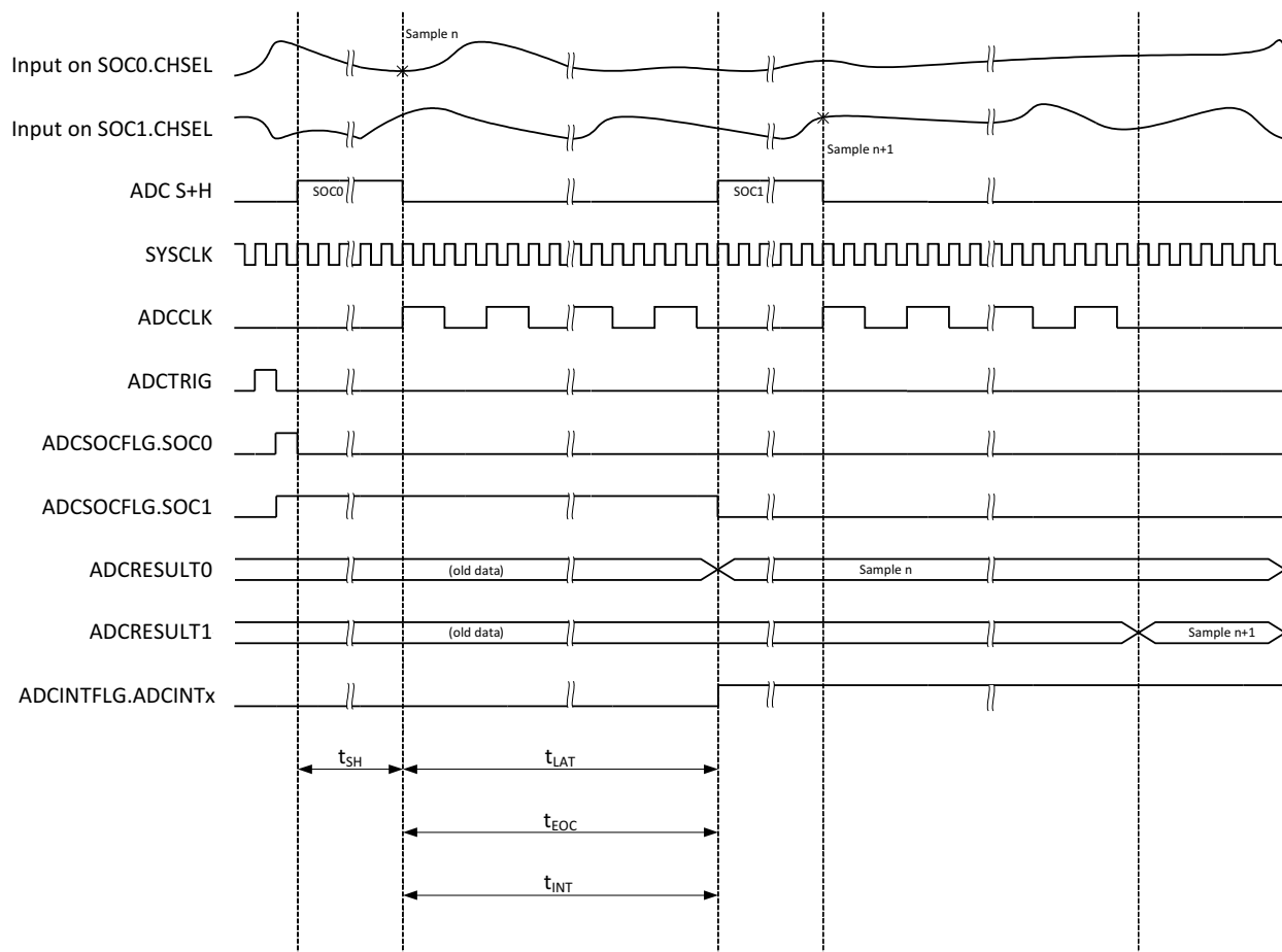
Figure 8-36. ADC Timings for 16-Bit Mode
