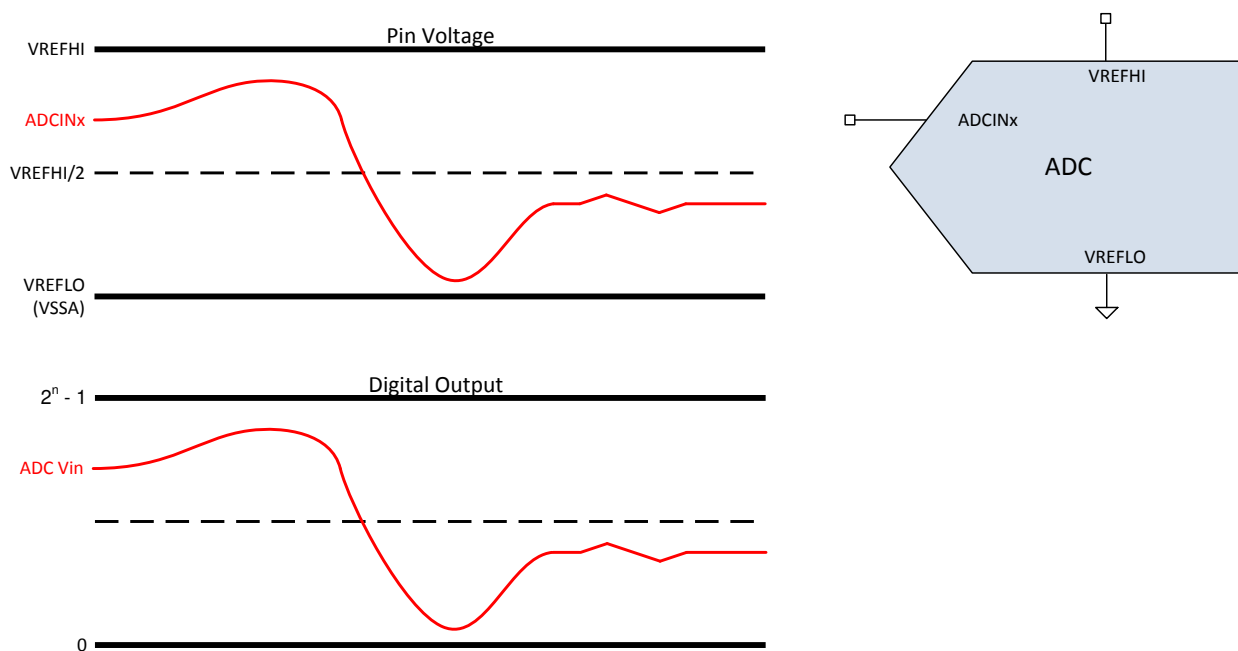
Figure 8-32. Single-ended Signaling Mode
