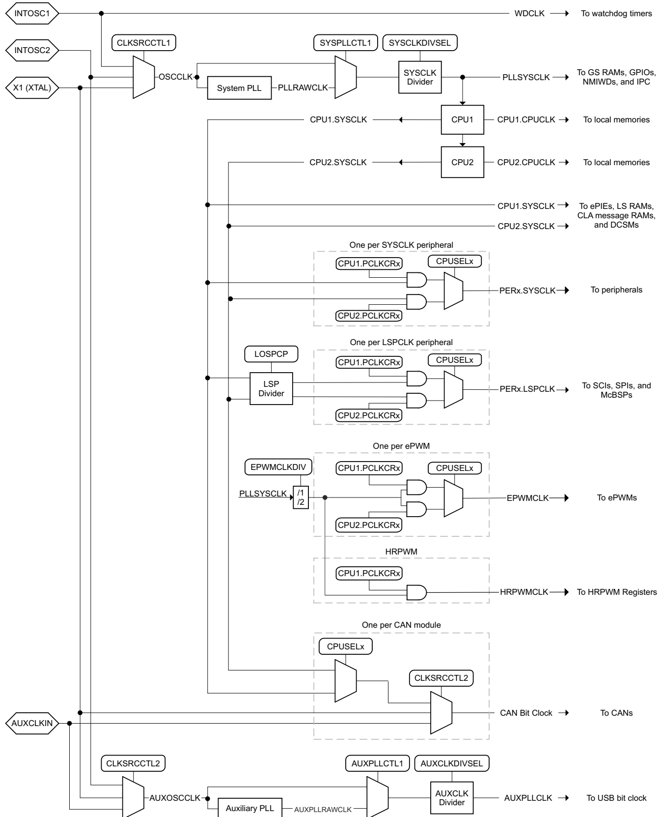
Figure 8-7. Clocking System
