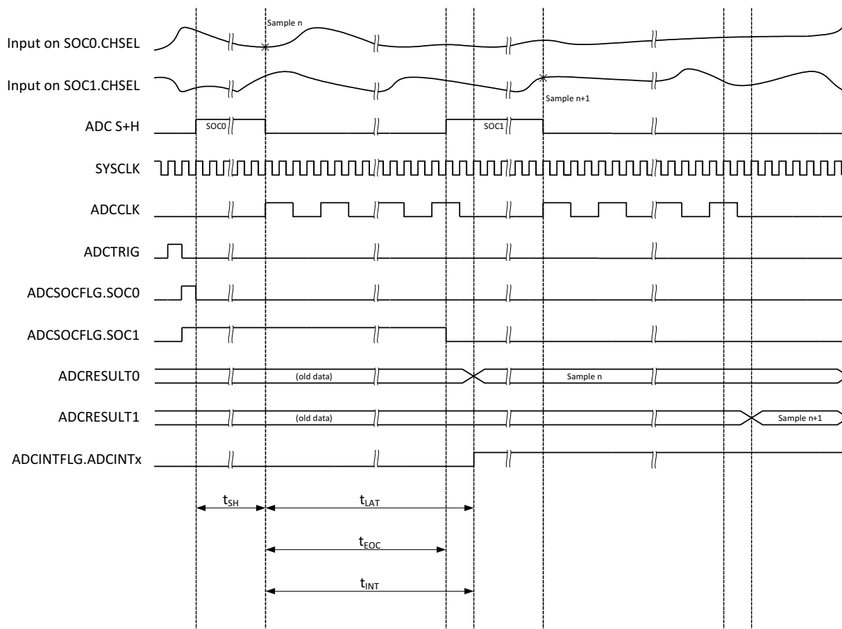
Figure 8-35. ADC Timings for 12-Bit Mode
