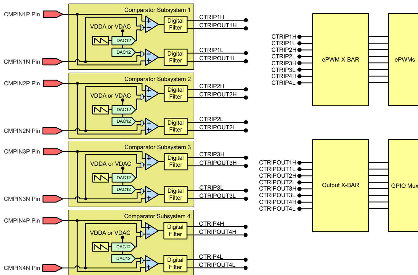
Figure 8-38. CMPSS Connectivity (100-Pin PZP)
