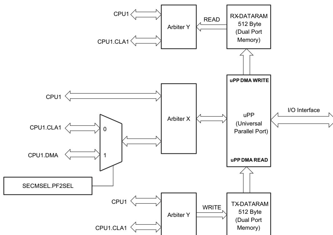
Figure 8-77. uPP Integration
