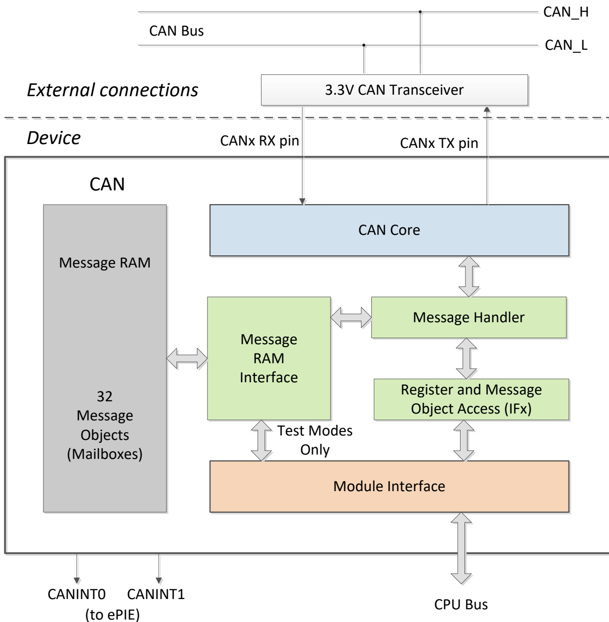
Figure 8-60. CAN Block Diagram
