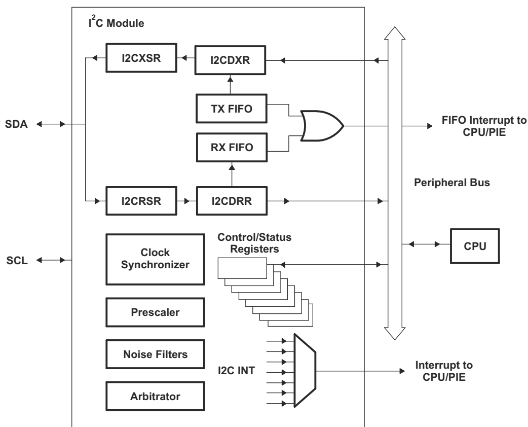
Figure 8-61. I2C Peripheral Module Interfaces
