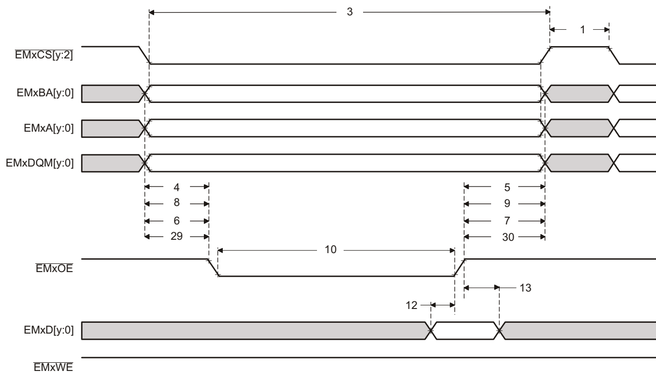
Figure 8-21. Asynchronous Memory Read Timing
