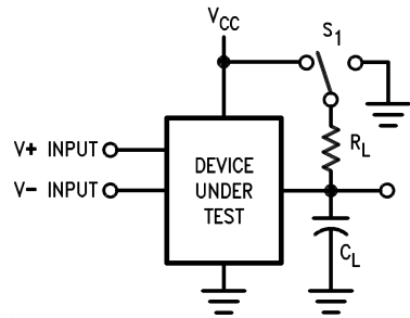
Figure 2. Propagation Delays
