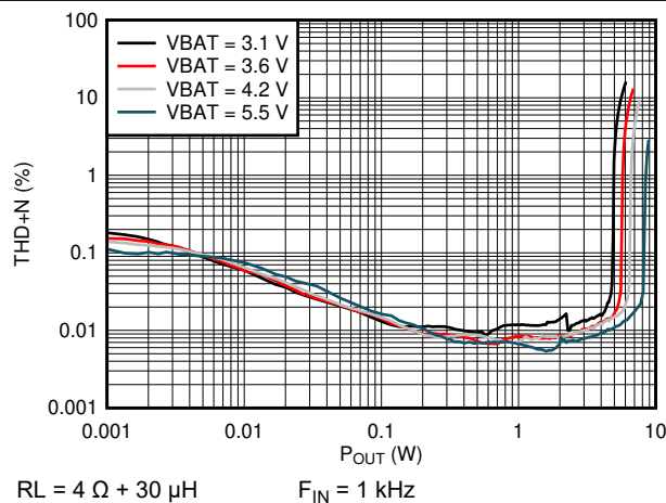
Figure 6-5. THD+N vs Output Power (DSBGA Package)
