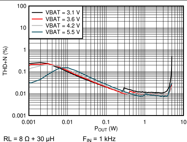
Figure 6-8. THD+N vs Output Power (QFN Package)
