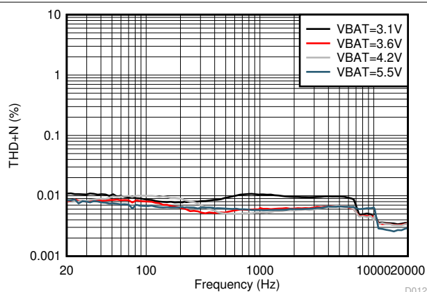
Figure 6-18. THD+N vs Frequency
