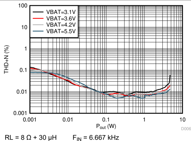
Figure 6-13. THD+N vs Output Power (DSBGA Package)
