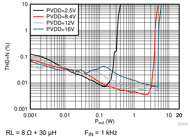
Figure 6-10. THD+N vs Output Power
