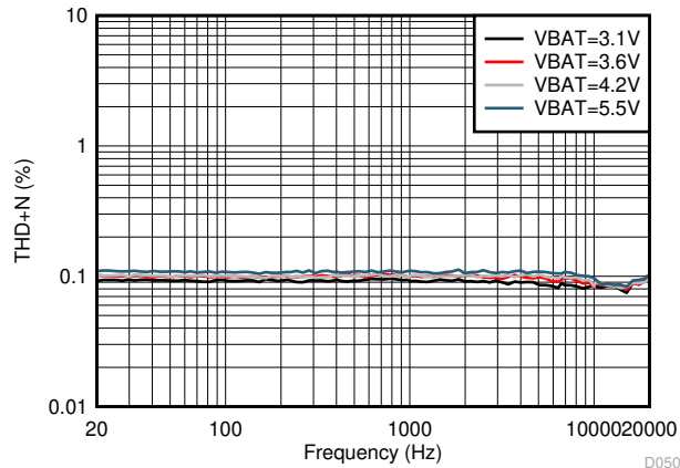
Figure 6-51. V-sense THD+N vs Frequency
