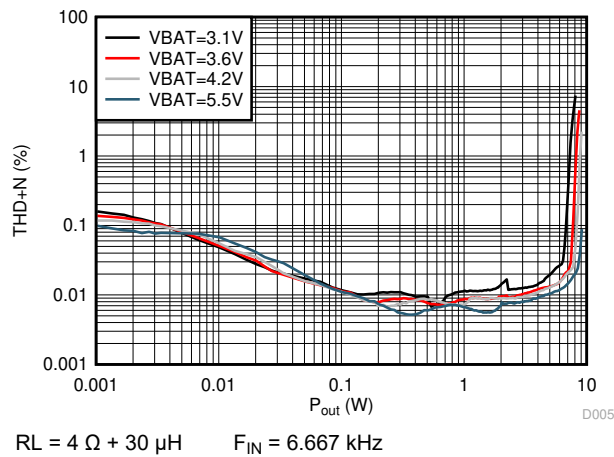
Figure 6-11. THD+N vs Output Power (DSBGA Package)
