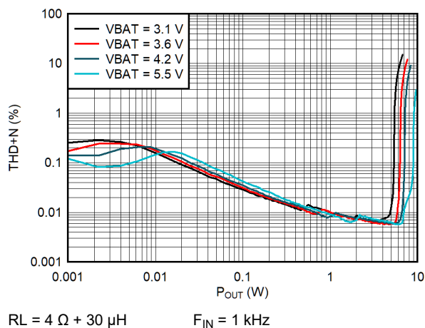
Figure 6-6. THD+N vs Output Power (QFN Package)
