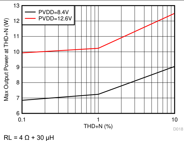
Figure 6-25. Max Output Power vs THD+N
