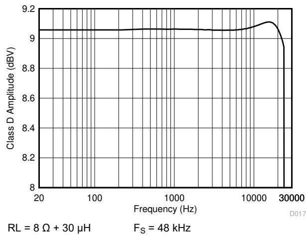
Figure 6-23. Amplitude vs Frequency
