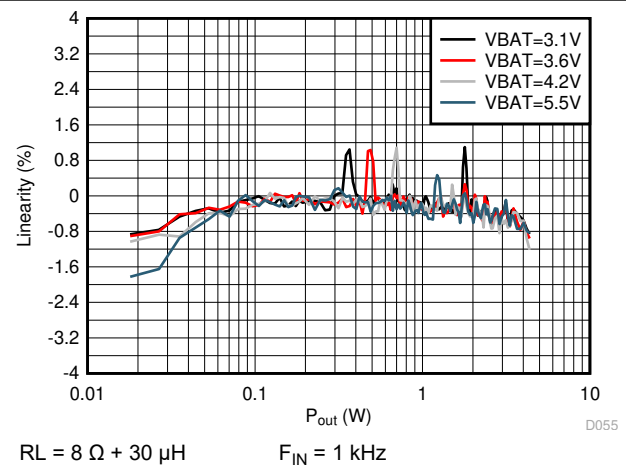
Figure 6-54. V/I-sense Linearity vs Output Power
