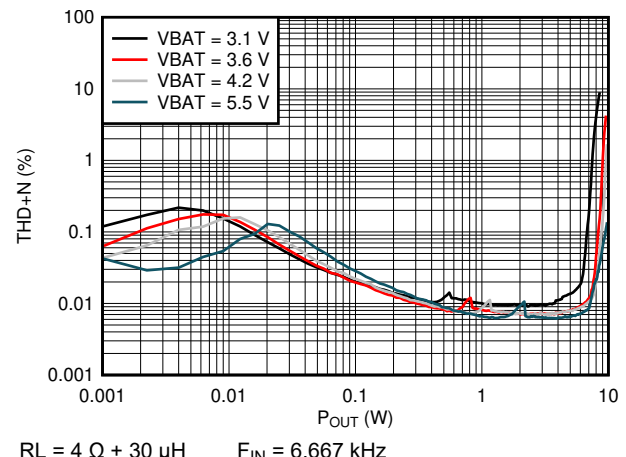
Figure 6-12. THD+N vs Output Power (QFN Package)
