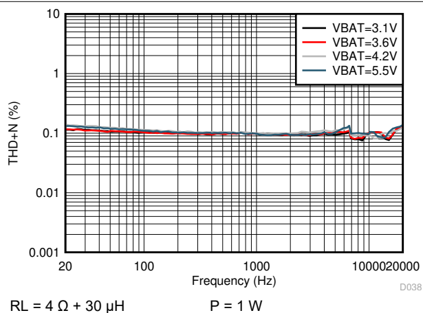
Figure 6-43. I-sense THD+N vs Frequency (DSBGA Package)
