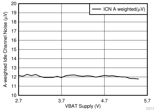
Figure 6-21. Idle Channel Noise (A-Weighted) vs VBAT
