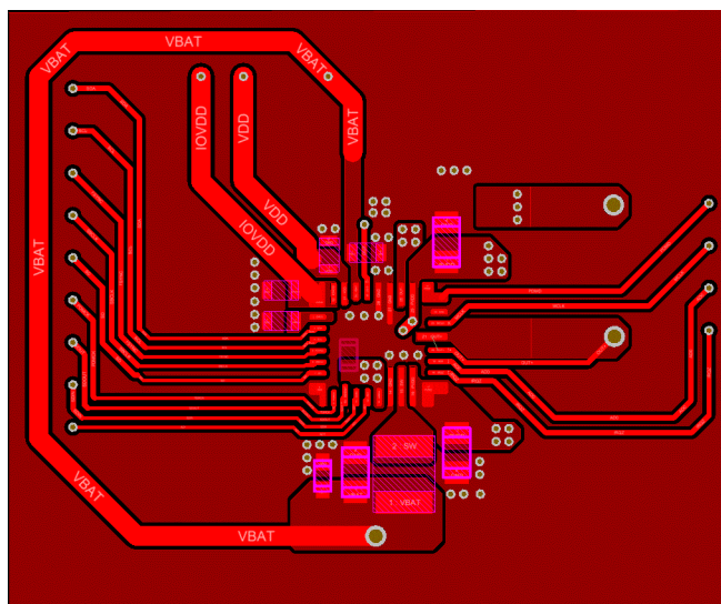
Figure 11-7. QFN Package Top Layer
