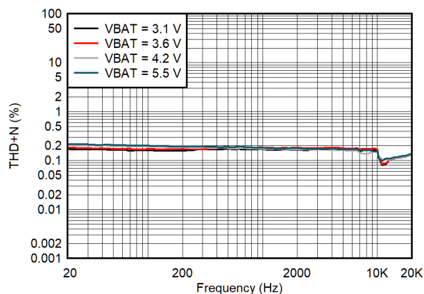
Figure 6-44. I-sense THD+N vs Frequency (QFN Package)
