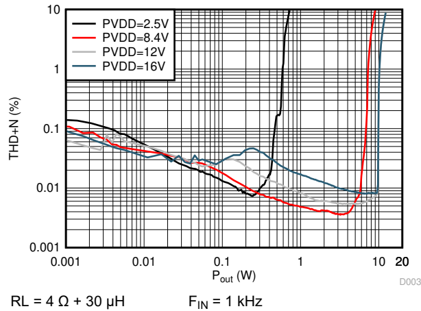
Figure 6-9. THD+N vs Output Power
