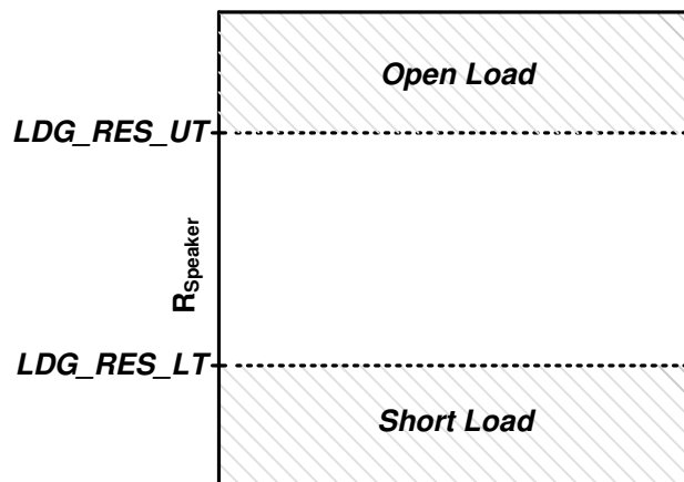
Figure 8-21. Load Diagnostics
