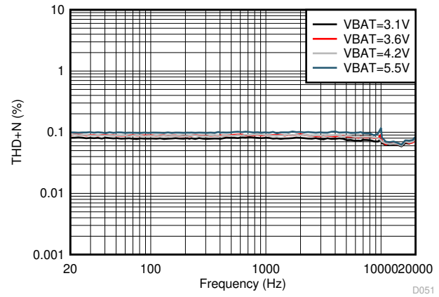
Figure 6-52. V-sense THD+N vs Frequency
