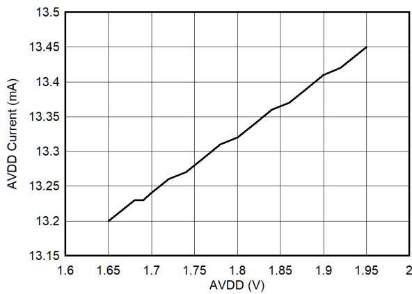
Figure 6-35. AVDD Idle Current vs AVDD (QFN Package)
