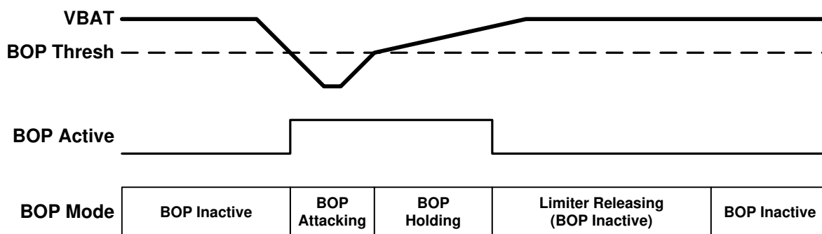
Figure 8-18. Brown Out Prevention Event
