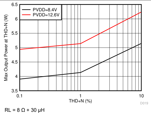
Figure 6-26. Max Output Power vs THD+N
