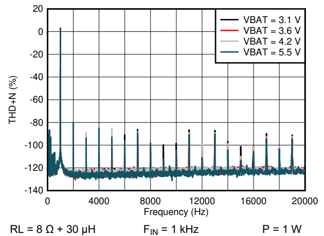
Figure 6-24. FFT Signal Plot
