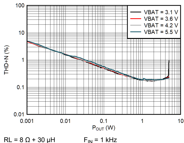
Figure 6-40. I-sense THD+N vs Output Power (QFN Package)
