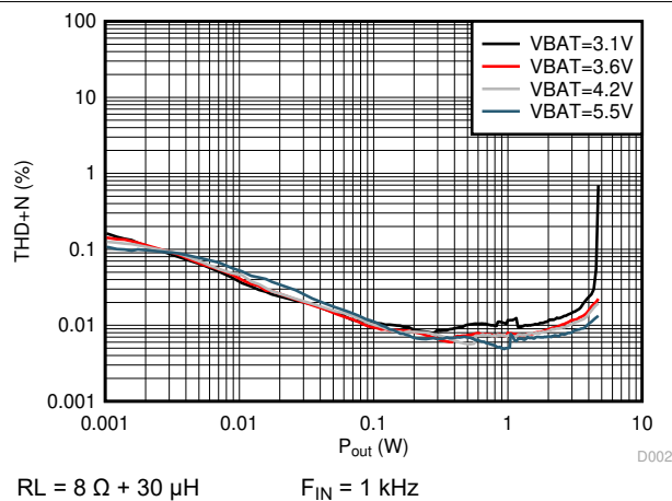
Figure 6-7. THD+N vs Output Power (DSBGA Package)
