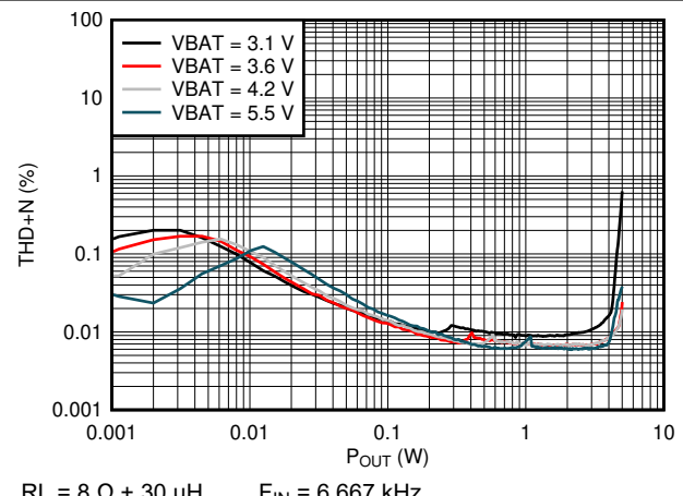
Figure 6-14. THD+N vs Output Power (QFN Package)
