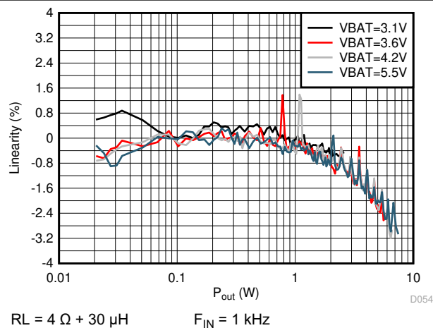
Figure 6-53. V/I-sense Linearity vs Output Power
