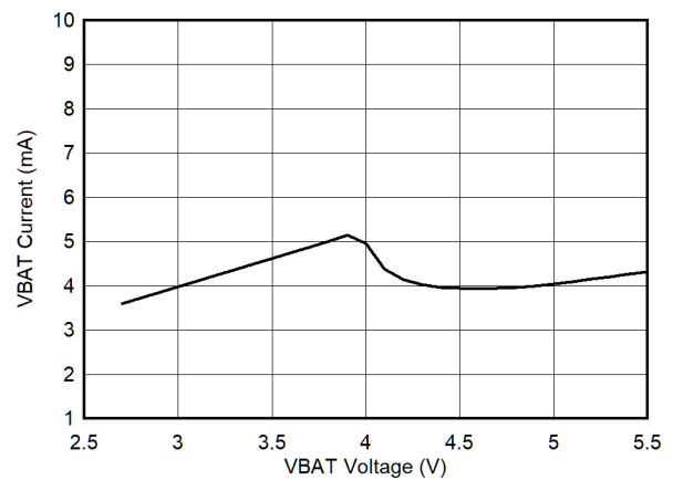
Figure 6-36. VBAT Idle Current vs VBAT
