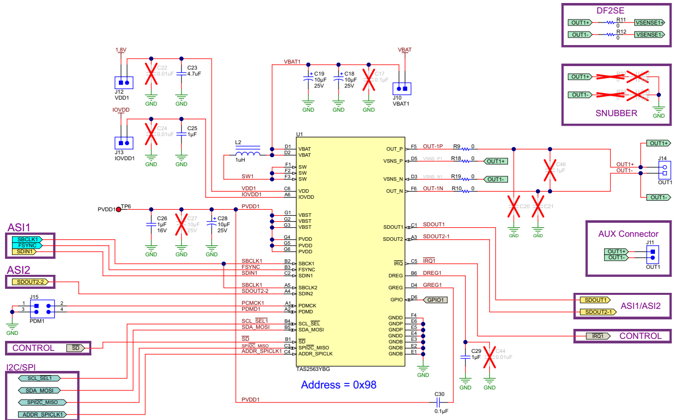
Figure 7-1. TAS2563 Circuit
