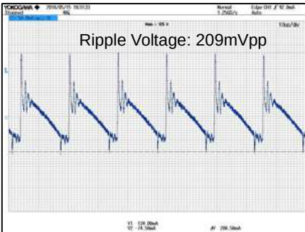
Figure 23. VOUT Ripple Voltage.6 V_{IN}=230Vac , I_{OUT}=1500mA CH1: VOUT 50mV/div, 10μs/div
