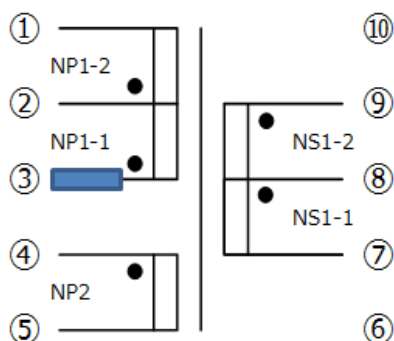
Figure 6. Connection Diagram
