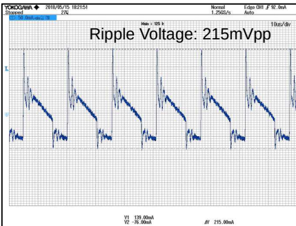
Figure 20. VOUT Ripple Voltage.3 V_{IN}=100Vac , I_{OUT}=1500mA CH1: VOUT 50mV/div, 10μs/div
