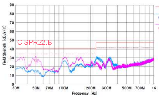
Figure 26. Radiated Emission.1
