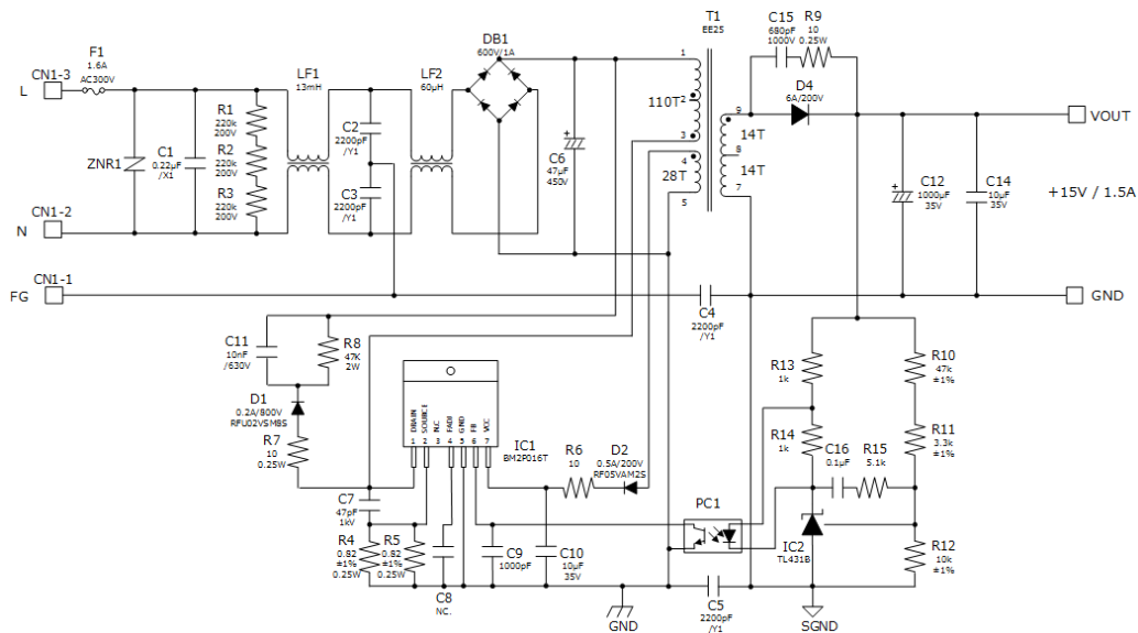
Figure 3. BM2P016T-EVK-002 Schematics
