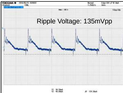
Figure 22. VOUT Ripple Voltage.5 V_{IN}=230Vac , I_{OUT}=500mA CH1: VOUT 50mV/div, 10μs/div
