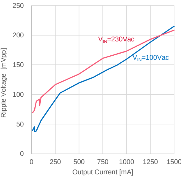
Figure 17. VOUT Ripple Voltage ( I_{OUT} vs. V_{ripple} )
