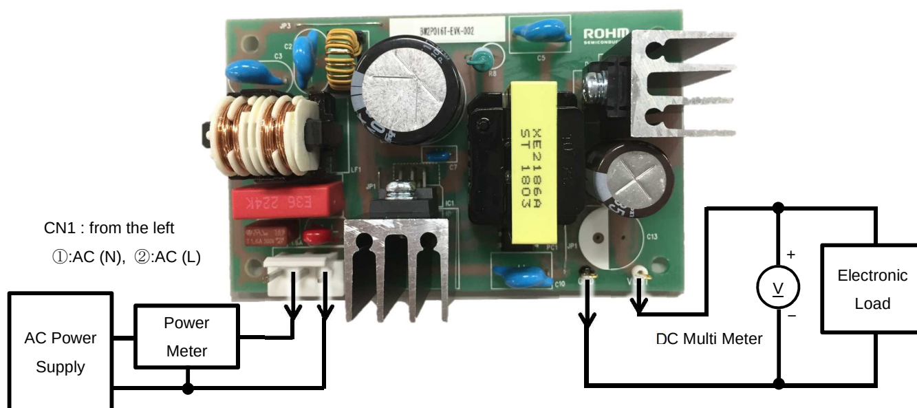
Figure 1. Connection Circuit
