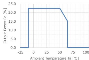
Figure 2. Temperature Derating curve
