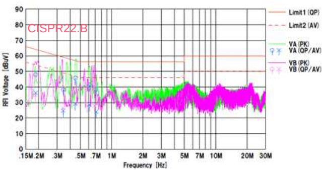
Figure 25. Conducted Emission.2
