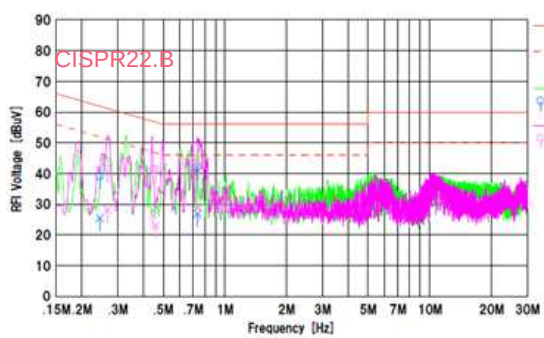
Figure 24. Conducted Emission.1
