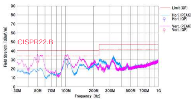
Figure 27. Radiated Emission.2
