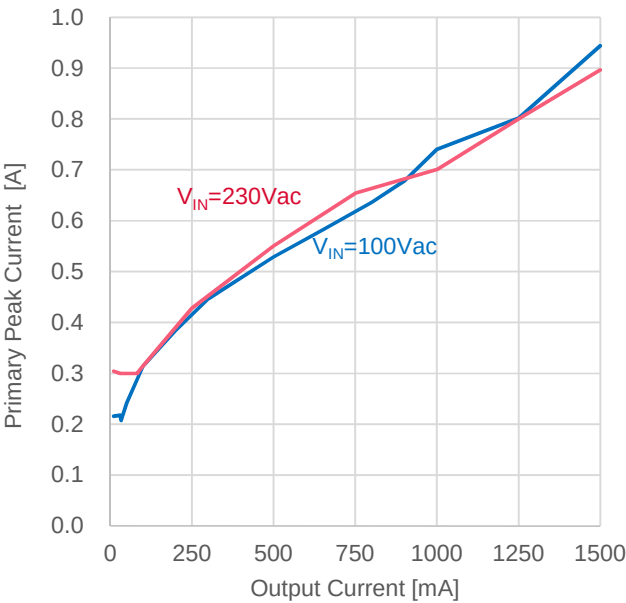
Figure 15. Primary Peak Current ( I_{OUT} vs. I_{peak} )
