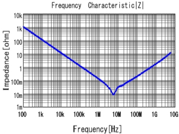
■ GRM188C70J225KE20 |Z| DC0V, 25degC
