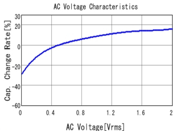
■ GRM188C70J225KE20 C-AC Voltage capchange, DC0V, 25.0d
