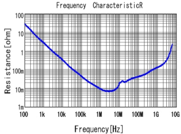
■ GRM188C70J225KE20 R DC0V, 25degC
