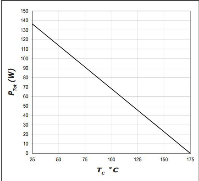
Figure 4 Power Derating
