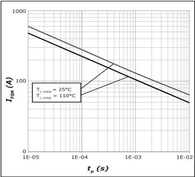
Figure 8 Non-Repetitive Peak Forward Surge Current versus Pulse Duration (sinusoidal waveform)
