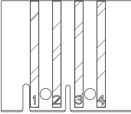
LAYOUT FOR CONNECTOR NO. 0-1740533-4 (WITHOUT PAD 2) 2-1740533-4
