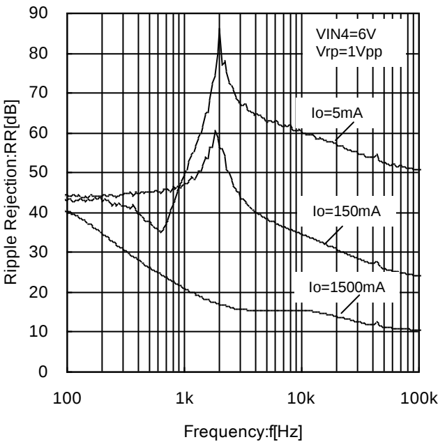
Figure 43. REG4 Ripple Rejection vs Frequency
