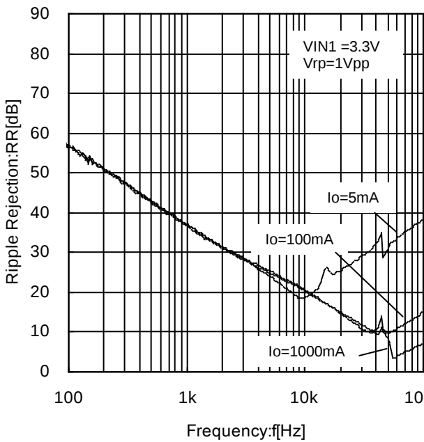
Figure 31. REG1 Ripple Rejection vs Frequency
