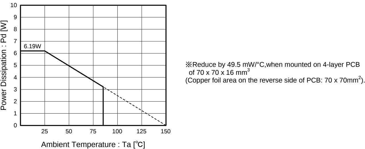
Figure 66. Thermal Reduction Characteristics
