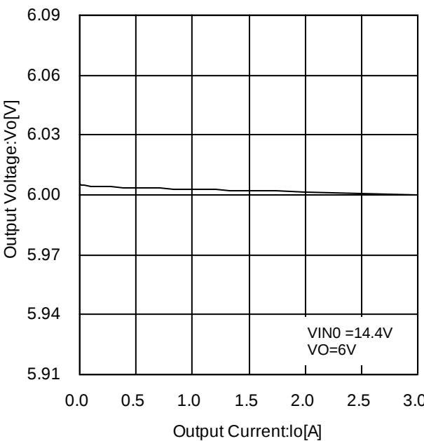
Figure 19. DCDC1 Output Voltage vs Output Current
