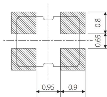
Figure 2) Land Pattern
