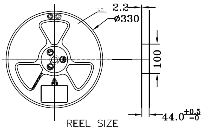
Figure 10.2. Reel Dimensions
